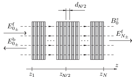
FIG. 1. The nonlinear magneto-optical crystal in the Faraday configuration. The setup consist of N - 1 layers of alternating optical and magneto-optical properties, with the centermost layer possessing twice the thickness of other layers with identical material properties.
