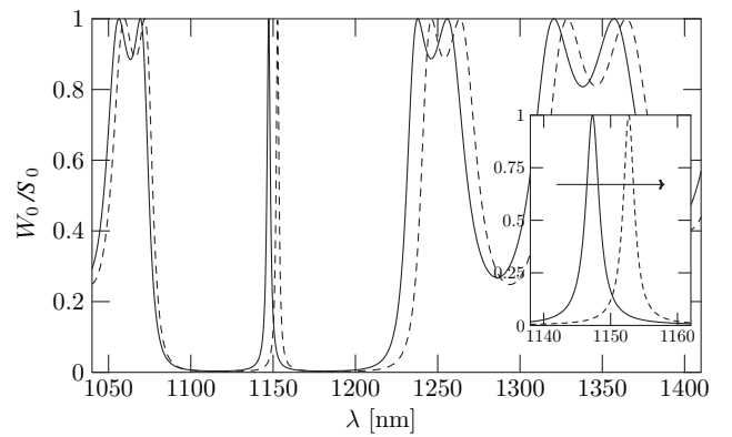
FIG. 2. Linear optical transmission for RCP (solid line) and LCP (dashed line) states of the incident optical wave vs vacuum wavelength \lambda = 2\pi c/\omega , for refractive index n_o = 2.18 and gyration coefficient g_o = 9.6 \times 10^{-3} of all odd layers. The corresponding parameters for even layers are n_e = 1.93 and g_e = 0 . The arrow in the inset graph shows the direction of displacement of the doublet of resonance peaks as the crystal is exposed to an intense light beam.
