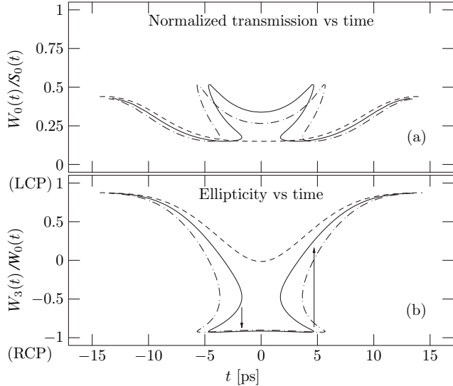
FIG. 3. The (a) normalized intensity transmission W_0/S_0 and (b) corresponding normalized ellipticity W_3/W_0 of the transmitted polarization state, as a function of time t for a linearly polarized input Gaussian pulse of half-maximum duration 10 ps and peak intensity 1.4 GW/cm 2 (dashed curves), 1.9 GW/cm 2 (solid curves), and 2.5 GW/cm 2 (dot-dashed curves). For a beam focused onto a spot of 40 \mu m diameter, the curves correspond to pulse energies of 190 nJ, 255 nJ, and 340 nJ, respectively.
