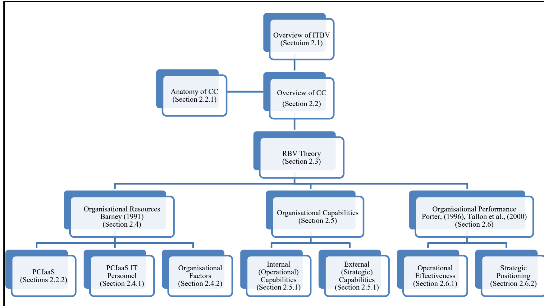
Figure 2-1: Research Structure
