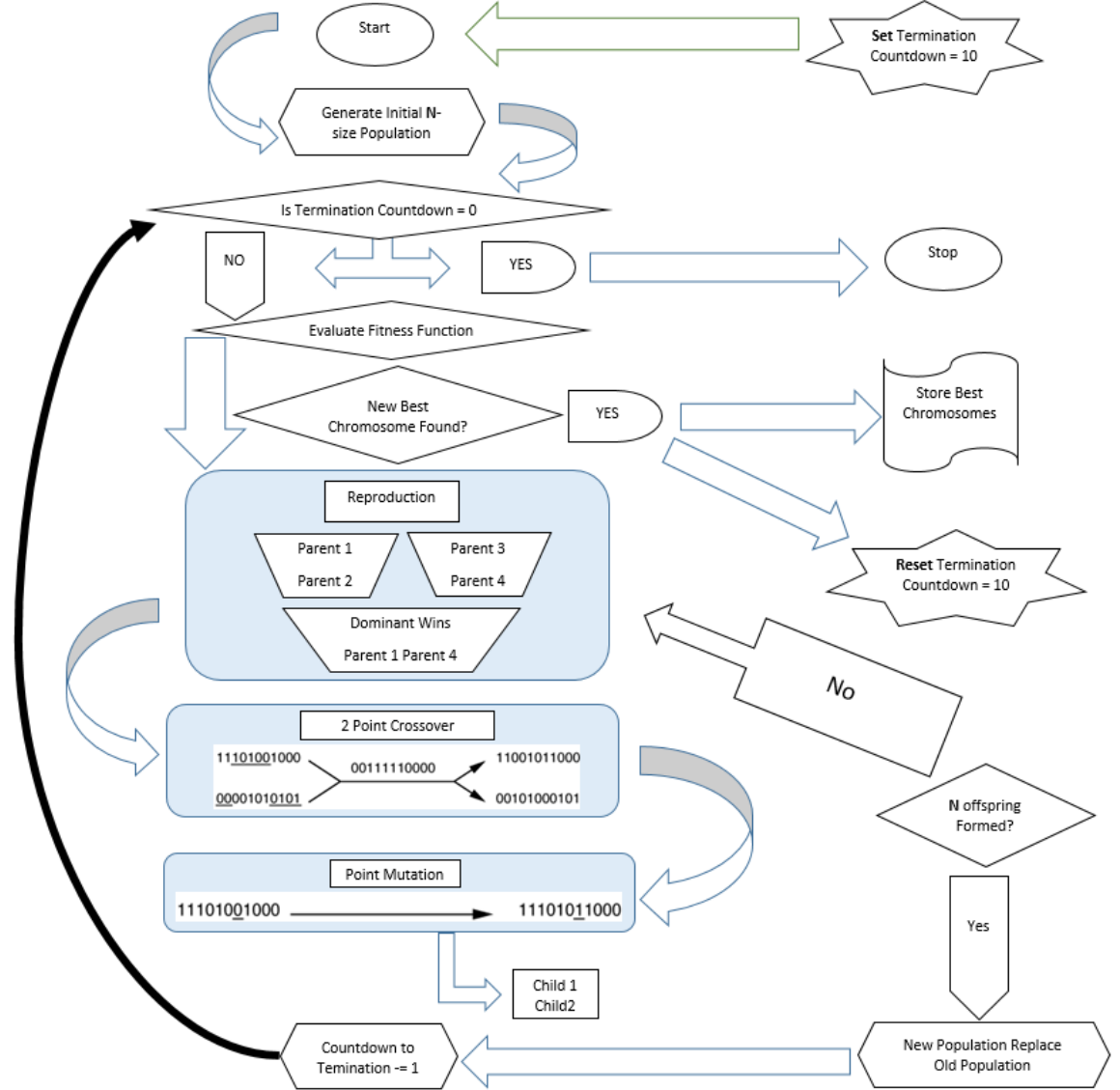
Figure 4.4: A diagram showing the flow of the proposed Genetic Algorithm.
