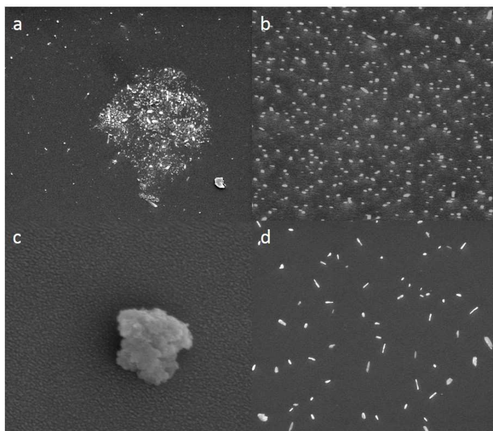
7 Fig. 2 SEM micrograph of native low molecular weight chitosan (a), 0.1 % w/v chitosan 8 nanoparticles (b), untreated 0.5 % w/v chitosan nanoparticles (c) and tip sonicated treated 0.5 % w/v 9 chitosan nanoparticles
