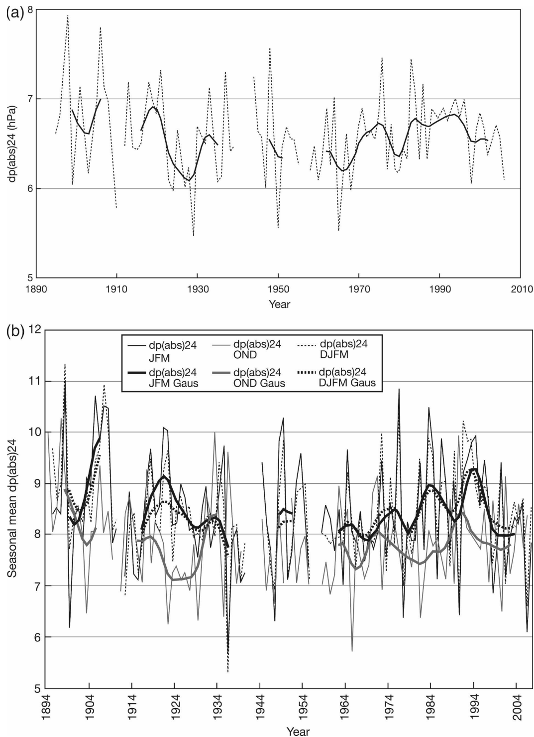
FIG. 8. (a) Tasiilaq (Greenland) annual dp(abs)24 with 21-point Gaussian filter, 1895–2006. There is a lack of data in the period September 1910–August 1911 and again from June 1940–January 1944—the latter because of the Second World War; (b) autumn, winter, and extended winter (DJFM) seasonal mean dp(abs)24 at Tasiilaq (Greenland), all with 21-point Gaussian filter, 1895–2007.
