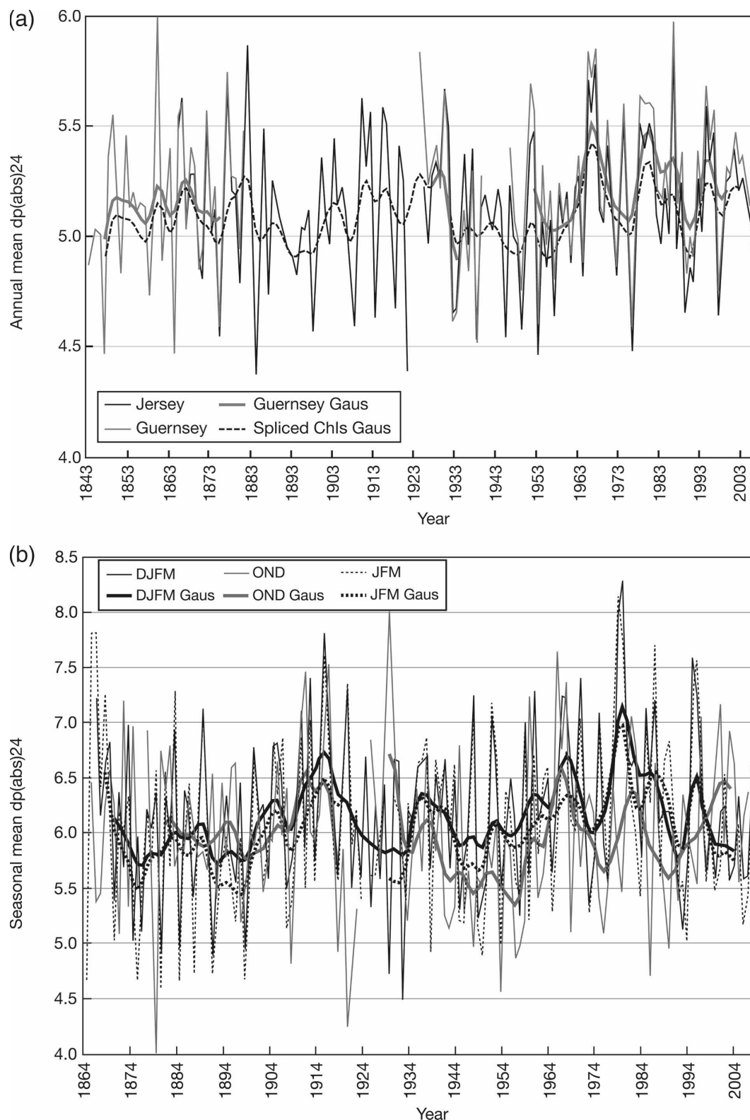
FIG. 6. (a) Annual mean dp(abs)24 at Jersey and Guernsey. The dashed curve is the 21-point, Gaussian-smoothed spliced Channel Islands annual dp(abs)24 series. The thick solid curve is the 21-point, Gaussian-smoothed Guernsey annual dp(abs)24 series. All are from 1843–2006; (b) autumn, winter, and extended winter (DJFM) seasonal mean dp(abs)24 at Jersey (U.K.), all with 21-point Gaussian filter, 1864–2007.
