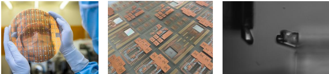
Figure 2: Novel glass interposer technologies for wafer-level scale up of PIC packaging developed in the PhotonicLEAP project: (a) full wafer (b) detailed view. (c) beam-steering fiber (left) to PIC (right) optical interconnect using 3D printed micro-optics
