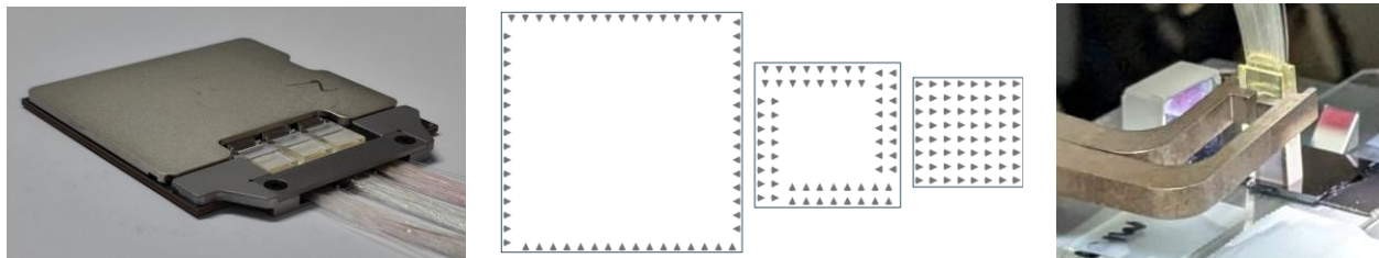
Figure 1: (a) Edge-coupled FPGA multi-chip package with three 56-channel FAs attached to one side (b) Illustrated on-chip area reduction for one-line, two-line, and 2D matrix optical coupler arrays. (c) A demonstrator package for a 96 channel ultra-fine pitch two-line fiber array.
