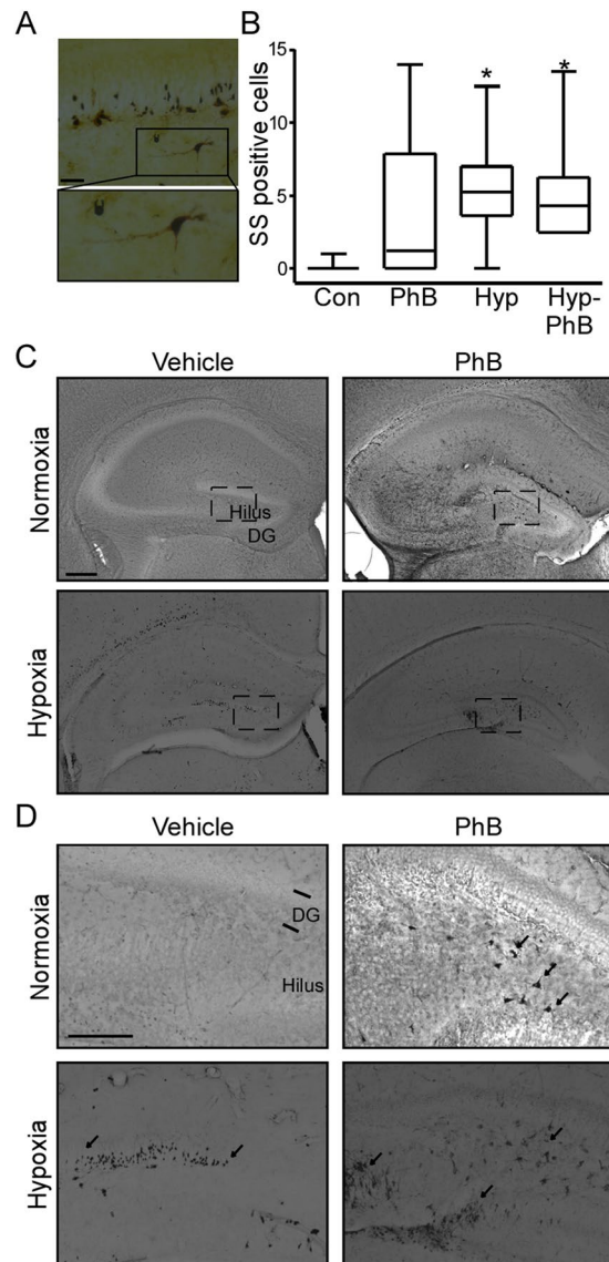
Figure 2. Neuronal damage after hypoxia-induced seizures in mice with/without phenobarbital (PhB) treatment at P7. (A) Representative high magnification (40x) silver staining images from the hypoxia group. Scale bar: 50 μm. (B) Graph shows the number of silver-staining positive cells. Note: Both hypoxia-exposed groups have more silver-staining positive cells ( n = 7 , *p < 0.05 compared to control). (C) Representative silver staining images of the hippocampus 72h post-treatment. Note: Silver staining positive cells were mainly observed in the hilus of the phenobarbital, hypoxia and hypoxia-PhB treated groups. Scale bar: 200 μm. (D) Representative images of the hilus area of control, phenobarbital and/or hypoxia exposed mice. Scale bar: 200 μm.
