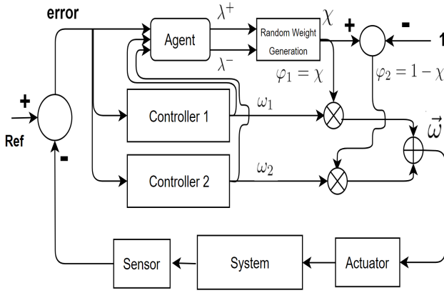
Fig. 1. The DRLRBC architecture (with two controllers).
