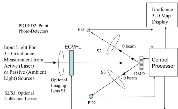
Figure 1. Proposed optical source 3D ( x , y , z ) irradiance-mapping instrument using a digital-mode digital-micromirror device (DMD) spatial sampler with an analog-mode electronically controlled variable-focal-length lens (ECVFL) with focus control. \pm\theta : Tilt angle.
