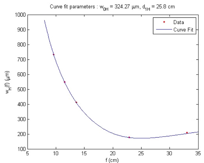
Figure 3. Experimental least-squares curve fit for the single-mode Gaussian laser based on the beam-waist parameters measured by the 3D irradiance system. w_H(f) : Minimum-beam waist in the horizontal direction ( x - y plane). d_{1H} : Relative location of the beam waist.
