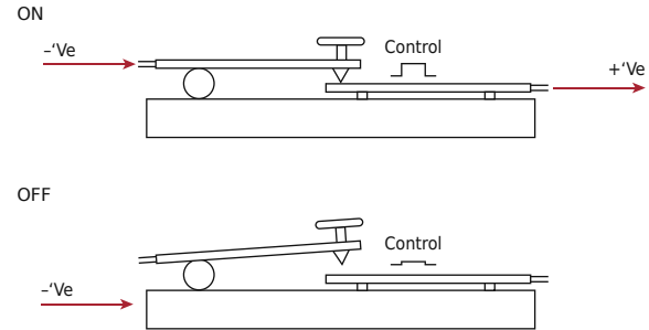
Figure 1. Morse code switch. Digital signals are switched between two states: ON and OFF. This can be done manually by using one's 'digit' or finger to make a connection. The result of the change of state is that current flows along the wire.
