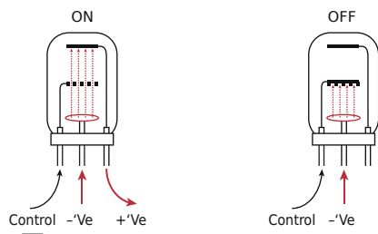
Figure 3. Electron Tube: Digital signals are switched between two states: ON and OFF. This can be done electronically by using a control current to permit the electron flow from the cathode (-ve) to the anode (+ve).
