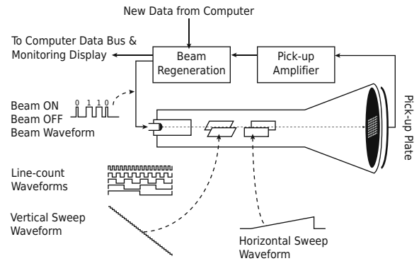
Figure 5. Williams-Kilburn tube Electrostatic Storage Memory. The Line-count and the Vertical Sweep waveforms control the position of the beam spot which is turned on or off by data from the computer. This places a grid of light spots on the screen which last for long enough to be re-generated; and if the Pick-up plate is removed an image can be displayed.
