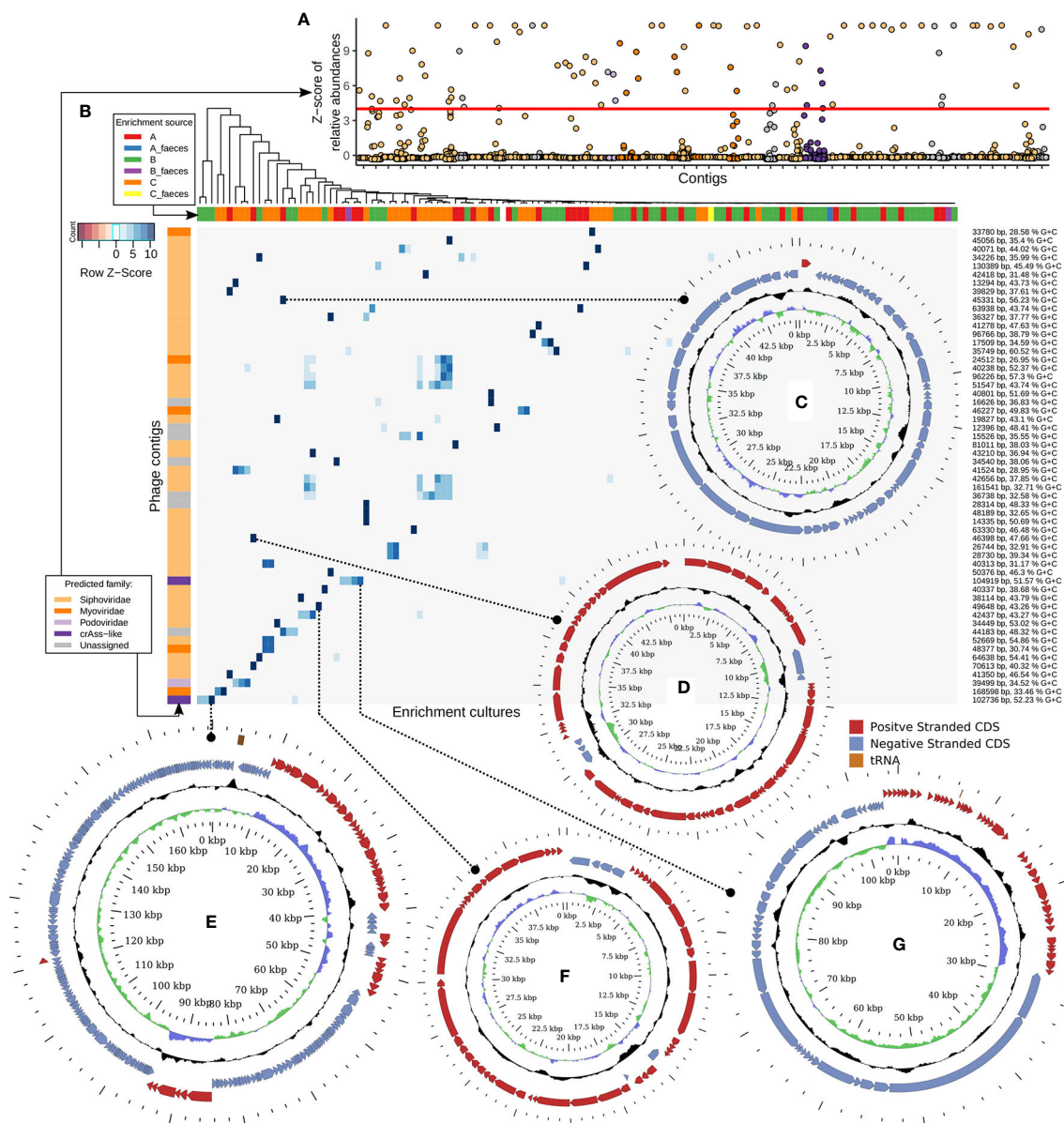
FIGURE 3 | Fifty six strongly enriched viral contigs represent diverse members of the order Caudovirales and replicated in the presence of typical human gut bacteria. (A) Z-scores of relative abundance of 56 manually selected viral genomic contigs across all study samples. Specific enrichment in one or a few related strains is a typical result. (B) Heatmap of scaled and centred relative abundance of 56 contigs across all 128 samples. (C) Circular genome of 35.3 kb Bacteroides uniformis DSM6597 phage; (D) circular genome of 46.4 kb temperate Siphoviridae phage infecting Anaerostipes hadrus APC942/1; (E) circular genome of a 168.6 kb E. coli phage; (F) circular genome of a 40.3 kb Subdoligranulum sp. APC924/74 inducible prophage; (G) circular genome of a 104.9 kb crAss-like phage of Prevotella stercora DSM 18206.
