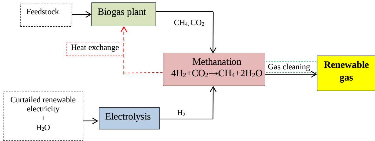
Figure 1: Design of biological P2G system as a biogas upgrading process
