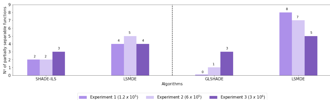
Fig. 10. Number of best partially separable functions. LSMDE vs SHADE-ILS and LSMDE vs GL-SHADE according to Conover post-hoc test for 1.2 \times 10^5 , 6 \times 10^5 and 3 \times 10^6 evaluations.
