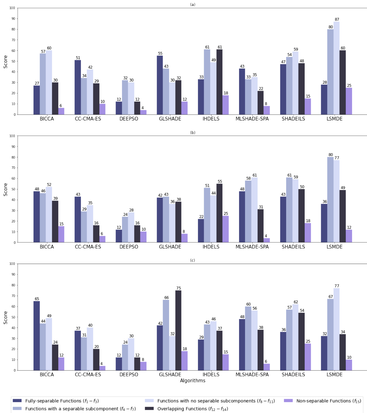
Fig. 7. Score of each competing algorithm based on the Formula One criterion for (a) 1.2 \times 10^5 , (b) 6 \times 10^5 and (c) 3 \times 10^6 evaluations of the objective function.
