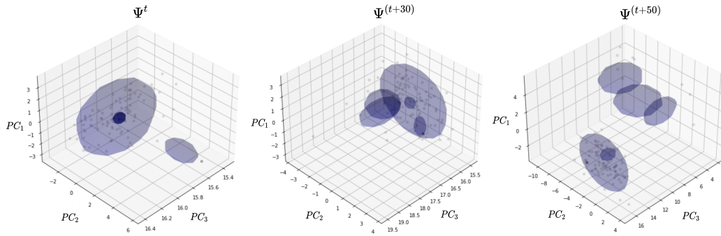
Fig. 4. Gaussian Mixture Models finding promising regions in the Alpine N1 low-dimensional search space. The number of clusters is automatically inferred by DP. In this case the number of clusters initially defined (population \Psi^t ) does not match the true generative distribution of the next populations; therefore, the Bayesian Gaussian mixture model fits the number of clusters according to the current population distribution.
