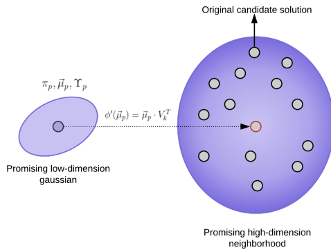
Fig. 5. Illustration of a space transformation from a promising Gaussian in \Psi to a promising region in \tilde{P} .
