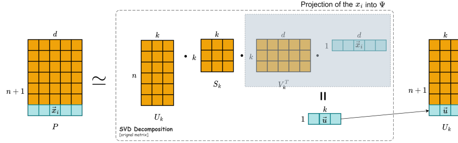
Fig. 3. Projection of a new high dimensional individual \vec{x}_i through the Low-rank approximation \phi(\vec{x}_i \in P) (folding-in)
