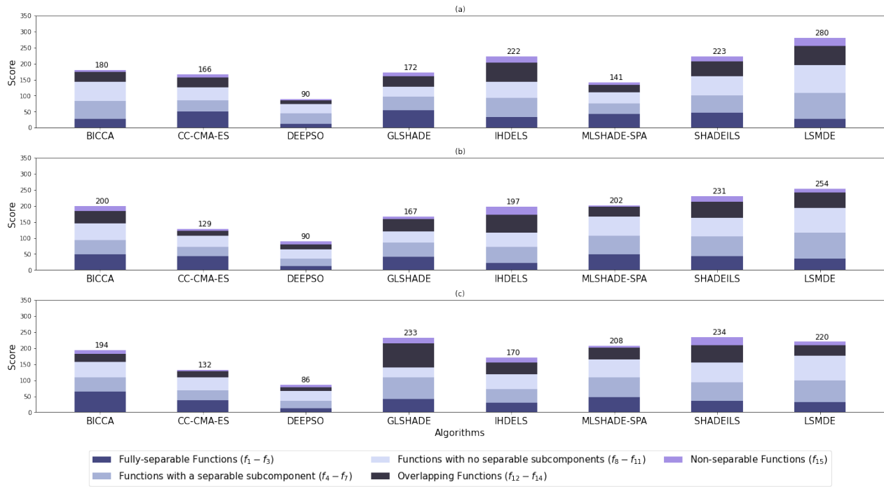
Fig. 8. General score based on the Formula One criterion for (a) 1.2 \times 10^5 evaluations, (b) 6 \times 10^5 evaluations and (c) 3 \times 10^6 evaluations.
