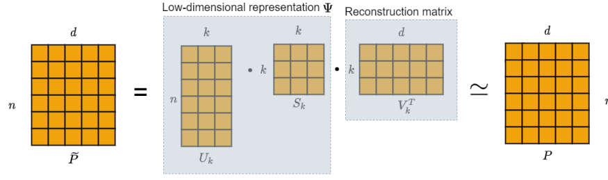
Fig. 2. Illustration of a low-dimensional representation from a d -dimensional random P matrix to a k -dimensional \Psi matrix.
