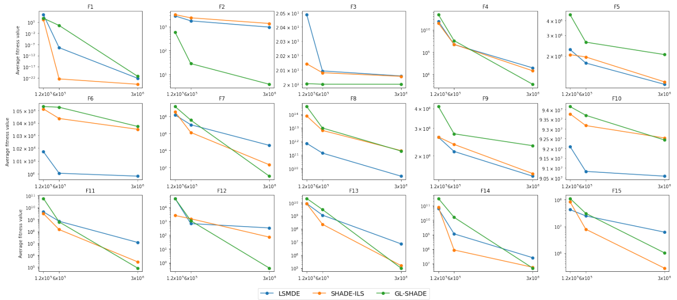
Fig. 9. Convergence functions of the three best competitor algorithms.
