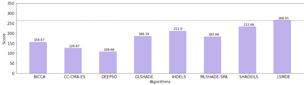
Fig. 6. Overall average score for 8 competitors based on Formula One criterion considering the three experiments. LSMDE has the best overall performance.
