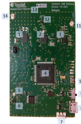
Figure 4. AUTHENTIC multiradio embedded system.
