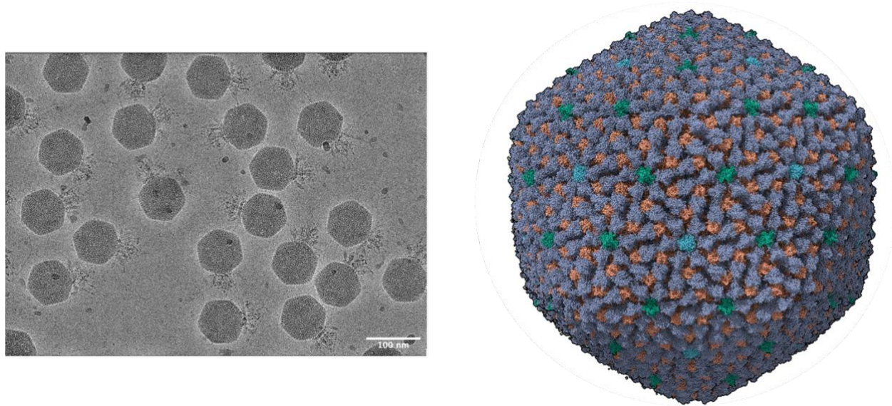
Figure 1. Overall structure of DAC15 capsid. A) Cryo-electron micrograph of DAC15 virions, n = 23,662 micrographs. B) Molecular surface of capsid reconstruction. The major capsid protein is coloured orange, auxiliary protein purple, head fibre dimer (residues 1-50) green and head fibre trimer (residues 1-39) blue.
