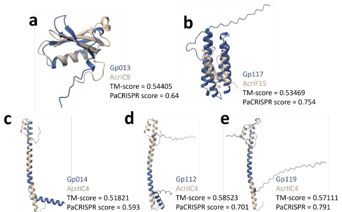
Figure 4. Predicted Acrs in DAC15 with structural similarity to experimentally determined Acrs.
