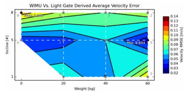
Fig. 13. RMSE of Sled Average Velocity for 2 Methods.
