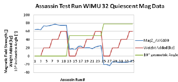
Fig. 21. Composite graph showing Magnetometer changes (Blue) for different Incline (Green) & Weight (Red) values.
