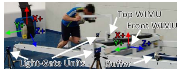
Fig. 3. Attached WIMU (inset) and Assassin In-Use.
