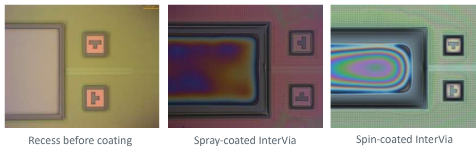
Figure 1. 120 \mu\text{m} wide and 2.5 mm long recess etched into a silicon photonics substrate before and after adhesive coating (spray / spin coat). Material piling at the edge of recess is visible under optical microscopy.
