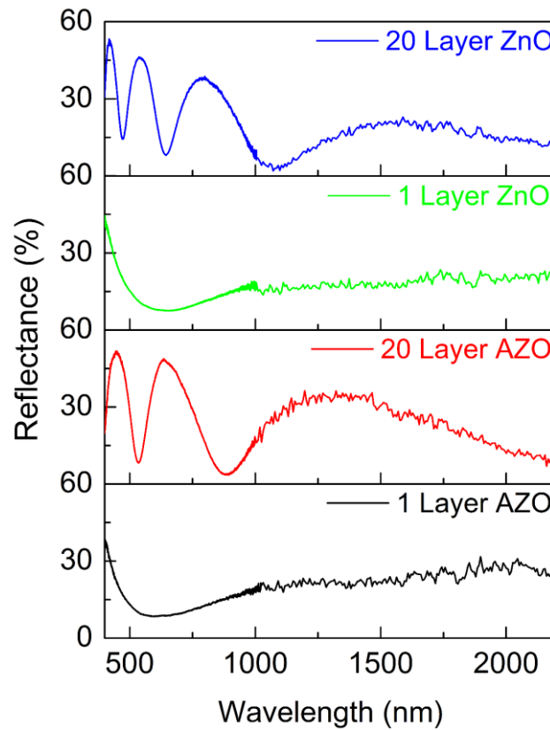
Figure 3. UV-vis-NIR reflectance spectra of single- and multi-layer ZnO and AZO thin films acquired at angle of incidence, \theta_i = 45^\circ .
