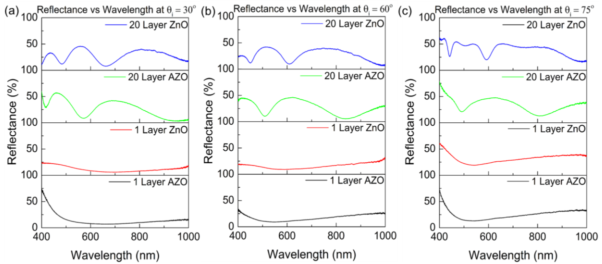
Figure 4. Angle dependent reflectance spectra of ZnO and AZO thin films acquired at various angles of incidence, \theta_i = (a) 30^\circ , (b) 60^\circ and (c) 75^\circ .
