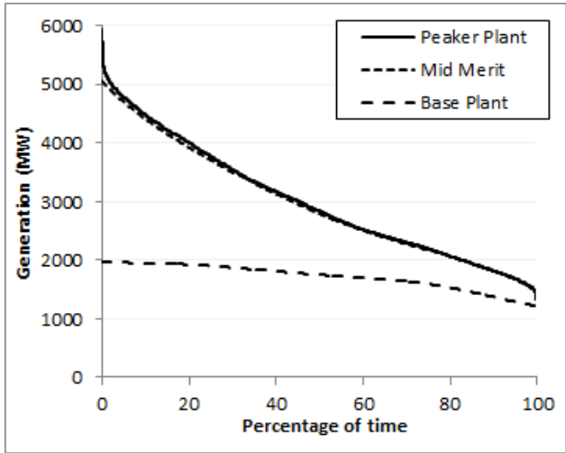
Figure 6: Load duration curves showing use of different conventional plant type for the medium offshore wind scenario excluding TCGs: (a) with an SNSP limit of 60%; (b) SNSP limit of 70%; & (c) SNSP limit of 100%.
