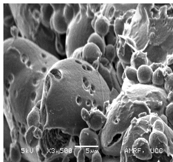
Figure 1.7: SEM: Endosperm of malted common wheat (magnification = 500x)
