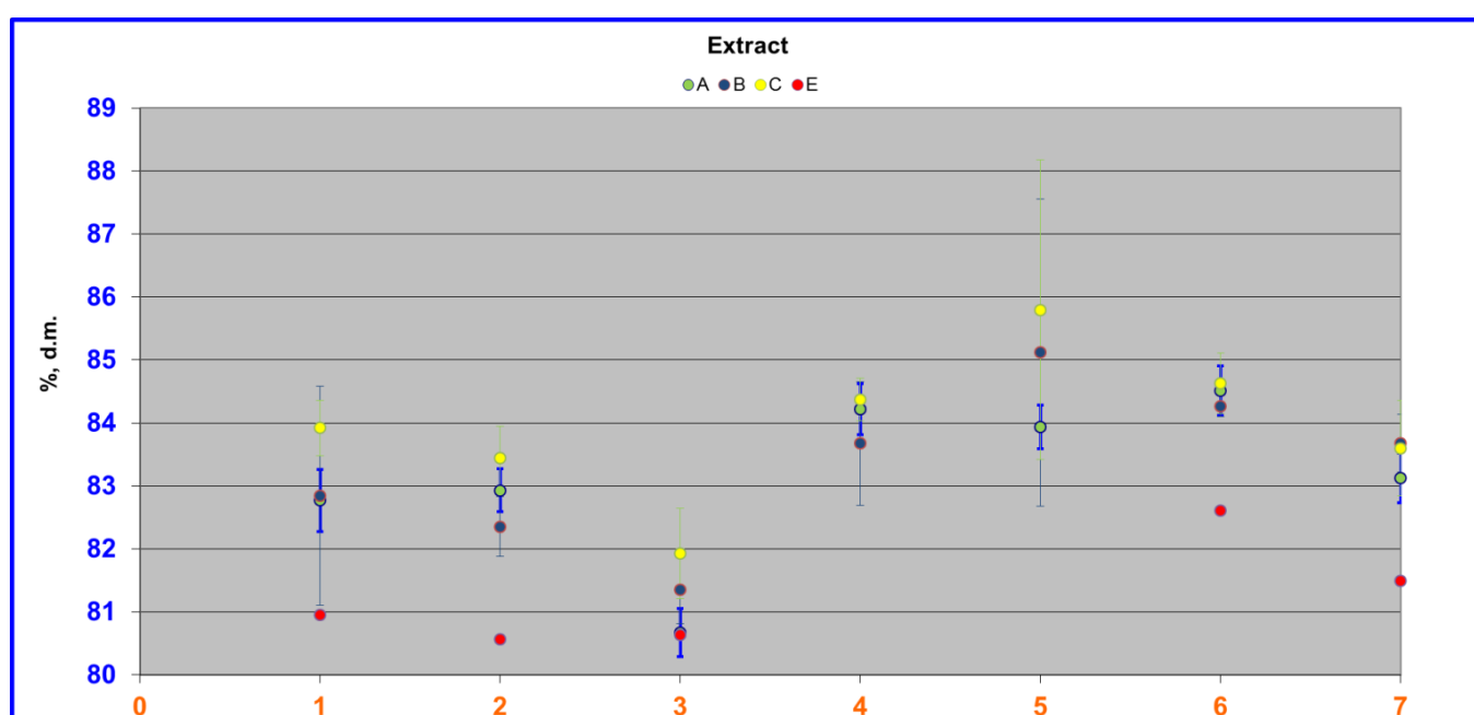
Figure 3.2: T-test distribution of extract values of different quality groups and growing region with a confidence interval of 95%, wheat quality groups according Table 3.1.
