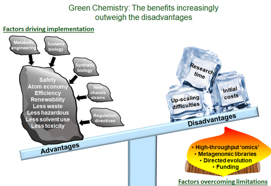
Figure 1. Green Chemistry: The Benefits Increasingly Outweigh the Disadvantages. Overview of the advantages and the disadvantages of green chemistry. Included are several solutions and strategies that combat the current disadvantages. These solutions and strategies include advancements in high-throughput screening, metagenomic library construction, directed evolution and funding opportunities.
