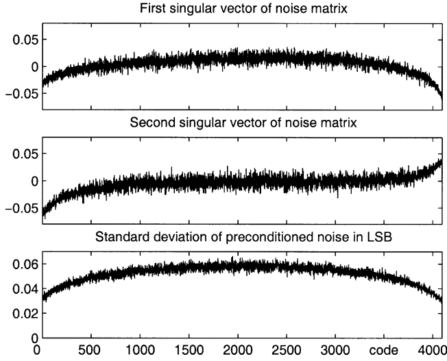
Fig. 4. First two singular vectors of measurement noise matrix (\tilde{B} - B) and standard deviation of \tilde{b}^* versus code.
