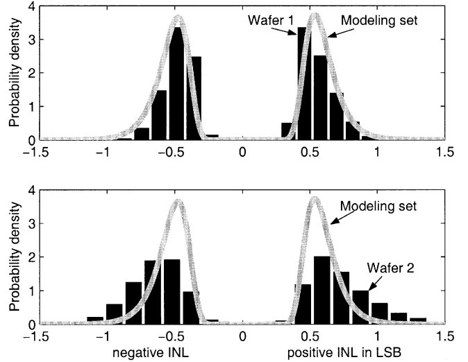
Fig. 5. Probability density versus INL performance for wafers 1 and 2 (shown as histograms) and for the modeling set (shown as a solid curve).
