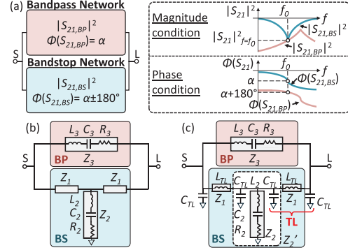
Fig. 1. (a) High-suppression BSF employing a two-path out-of-phase SC. (b) BTN implementation with generic Z_1 impedance. (c) Modification with \pi -type TL.
