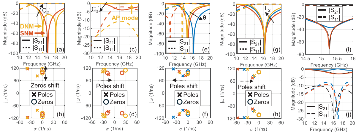
Fig. 2. (a) BSF mode S-parameters and (b) pole-zero plot for L_2 = L_3 = 0.563 nH, C_3 = 120 fF, R_2 = R_3 = 0 \Omega , Z_{0TL} = 50 \Omega , and \theta = 45^\circ : SNM ( C'_2 = 86.24 fF) and DNM ( C'_2 = 80 fF). (c) AP mode S-parameters and (d) pole-zero plot for L_2 = L_3 = 0.563 nH, C_2 = 120 fF, R_2 = R_3 = 0 \Omega , Z_{0TL} = 50 \Omega , \theta = 45^\circ , and C'_3 = 66, 105 fF. (e) SNM BSF mode S-parameters and (f) pole-zero plot for L_2 = L_3 = 0.563 nH, R_2 = R_3 = 0 \Omega , Z_{0TL} = 50 \Omega , and \theta variations: 10^\circ ( C_3 = 175 fF and C'_2 = 174.26 fF), 25^\circ ( C_3 = 147 fF and C'_2 = 139.07 fF), and 45^\circ ( C_3 = 120 fF and C'_2 = 86.24 fF). (g) SNM BSF mode S-parameters and (h) pole-zero plot for R_2 = R_3 = 0 \Omega , Z_{0TL} = 50 \Omega , and \theta = 45^\circ for: L_2 = L_3 = 0.2 nH ( C_3 = 190 fF and C'_2 = 100.95 fF), L_2 = L_3 = 0.563 nH ( C_3 = 120 fF and C'_2 = 86.24 fF), and L_2 = L_3 = 0.8 nH ( C_3 = 95 fF and C'_2 = 73.92 fF). BSF-to-AP S-parameters for L_2 = L_3 = 0.563 nH, R_2 = R_3 = 4 \Omega , Z_{0TL} = 50 \Omega , and \theta = 25^\circ for (i) SNM ( C'_2 = 139.07 fF) with C_3 = 147 fF (blue trace) and C'_3 = 145.63 fF (orange trace) and (j) AP mode ( C_2 = 147 fF) for C'_3 = 93 fF ( R_2 = R_3 = 0 \Omega , blue trace) and C'_3 = 93 fF ( R_2 = R_3 = 4 \Omega , orange trace). Black traces: circuit simulations.
