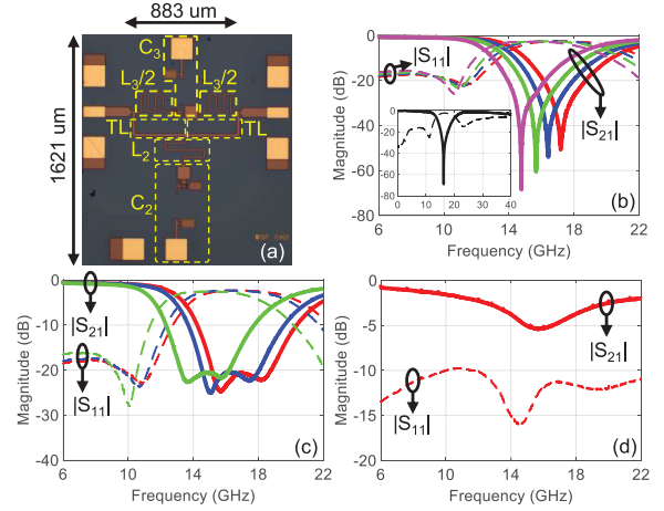
Fig. 3. BSF-to-AP. (a) Manufactured prototype with: L_2 = 0.536 nH, C_2 = 51\text{--}256 fF, R_2 = 4.83 \Omega , L_3 = 1.072 nH, C_3 = 75\text{--}267 pF, R_3 = 4.56 \Omega , Z_{0TL} = 73 \Omega , \theta = 25^\circ , C_{TL} = 47.05 fF, and L_{TL} = 0.224 nH. Measured S-parameters. (b) SNM. (c) DNM. (d) AP mode.
