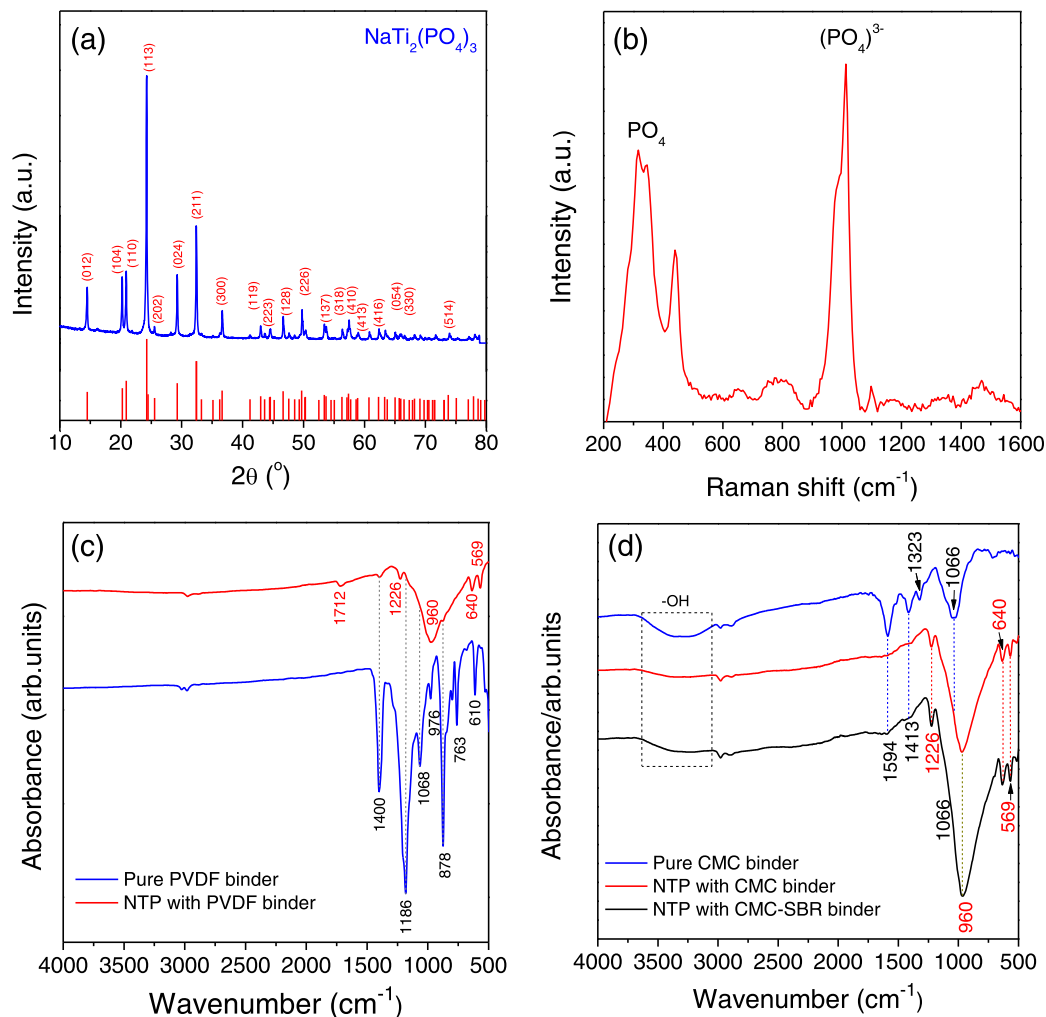
Figure 1. (a) X-ray diffraction pattern of the \text{NaTi}_2(\text{PO}_4)_3 anode material following hydrothermal synthesis. The reflections are indexed to the reference JCPDS file No. 00–033–1296. (b) Raman scattering spectra for NTP nanoparticulate material acquired under 532 nm excitation. (c) FTIR spectra of pure PVDF binder and the NTP electrode slurred with PVDF binder. (d) FTIR spectra of pure CMC binder and of the NTP electrode mixed with CMC and CMC-SBR binders.
