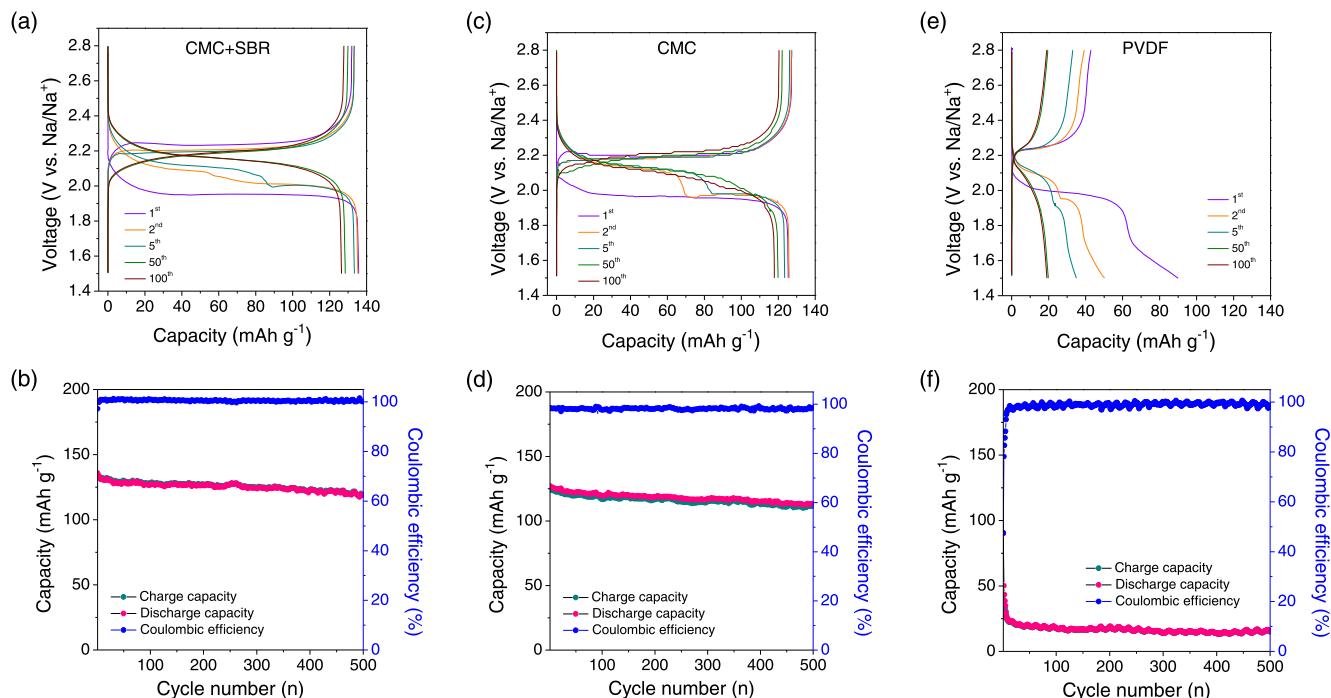
Figure 4. Galvanostatic charge-discharge curves and cycling stability tests for the \text{NaTi}_2(\text{PO}_4)_3 electrode slurries acquired at 0.2 C rate (capacity at 1 C = 133 \text{ mAh g}^{-1} ) over 500 cycles using (a), (b) CMC/SBR, (c), (d) CMC, and (e), (f) PVDF binders.
