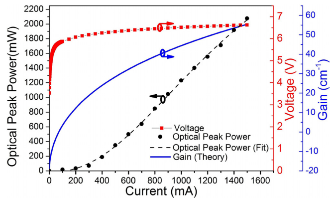
FIG. 2. Light-current-voltage characteristics of blue SLED under pulsed operation. Superluminescence is observed above 300 mA. Peak optical powers >2\ \text{W} are measured. The operating voltage of the device is between 6 and 7 V. Also shown is the extracted gain as a function of current.
