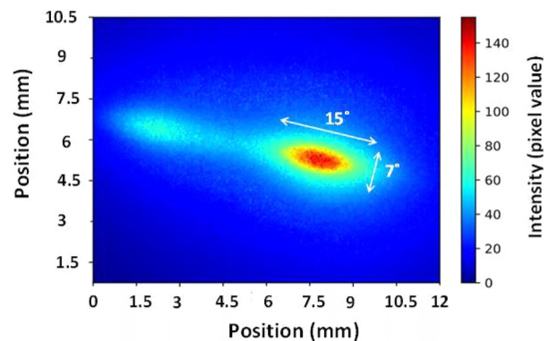
FIG. 3. Far field image of blue SLED at 500 mA. The divergence from a single output is measured to be 7^\circ \times 15^\circ .
