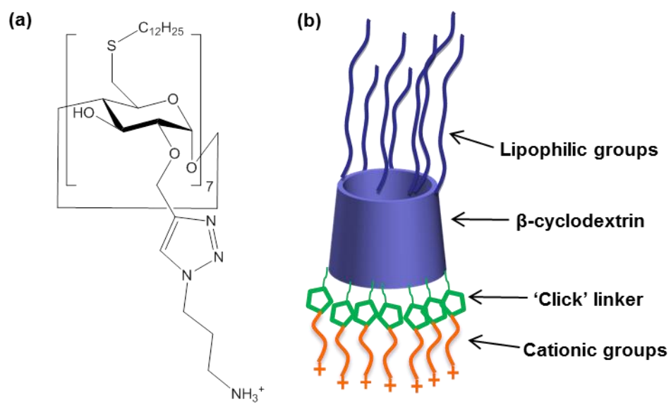
Figure 1. (a) Chemical structure of CD used for siRNA delivery and (b) schematic representation of CD structure.
