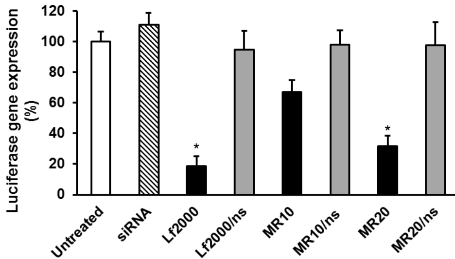
Figure 5. Knockdown of luciferase reporter gene in mHypoE N41 cells by CD.siRNA complexes. Cells were incubated with luciferase reporter plasmid (1 \mu g/well). Four hours later, after washing and changing media, luciferase siRNA (50 nM), either uncomplexed, or complexed to CD, was added. After 24 hours, reduction in gene expression was measured by luciferase assay. Data (n=3) are expressed as the mean \pm SEM. * p < 0.05 relative to untreated controls.
