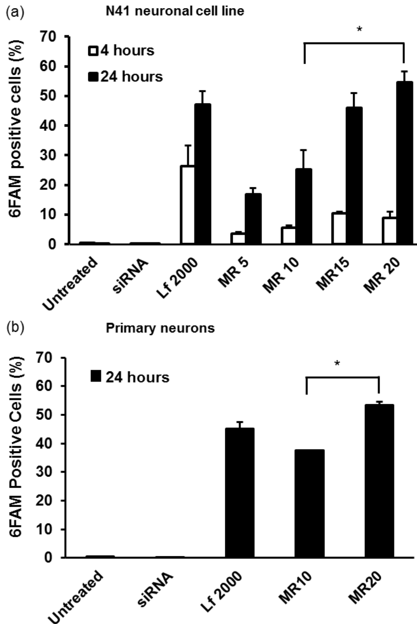
Figure 4. Internalisation of CD.siRNA complexes by (a) mHypoE N41 cells and (b) Primary rat (E18) hippocampal cells. FAM-siRNA uptake, after incubation with CD.siRNA complexes (siRNA 50 nM), was measured by flow cytometry. Data (n=3) are expressed as the mean \pm SEM. * p < 0.05 relative to untreated controls.
