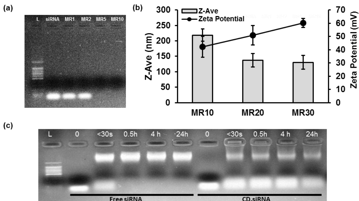
Figure 2. Properties of CD.siRNA complexes. (a) CD.siRNA binding was shown by gel electrophoresis. Fluorescent bands correspond to 100 b.p. DNA ladder (L), free siRNA and unbound siRNA. (b) Z-Ave (size, (nm)) and Zeta Potential (charge, (mV)) of CD-siRNA complexes at increasing mass ratios (MR; \mu\text{g CD} : \mu\text{g siRNA} ), were measured in DIW (final siRNA concentration 3 \mu\text{g/ml} ), using dynamic light scattering (Malvern ZetaSizer Nano). (c) Serum degradation assay, as shown by gel electrophoresis. Uncomplexed siRNA or CD.siRNA was exposed to 50% serum for up to 24hours. CD at least partially protected siRNA from degradation.
