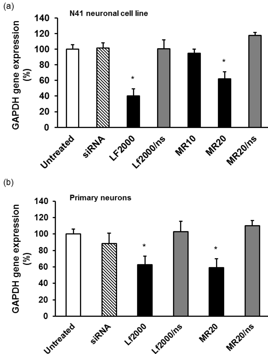
Figure 6. Knockdown of endogenous GAPDH in (a) mHypoE N41 cells and (b) Primary rat (E18) hippocampal cells by CD.siRNA complexes. Cells were incubated GAPDH siRNA (100 nM), either uncomplexed, or complexed to CD, for 24 hours. Total RNA was extracted and reverse transcribed to cDNA for qRT-PCR, to determine the reduction in GAPDH mRNA expression. Data (n=3) are expressed as the mean \pm SEM. * p < 0.05 relative to untreated controls.
