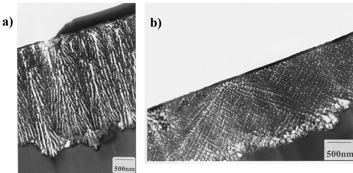
Fig. 6 (a) Bright field TEM of InP after a potential sweep from 0.0 V to 0.825 V (SCE) in 2 \text{ mol dm}^{-3} KOH (b) Bright field TEM of InP after a potential sweep from 0.0 V to 0.675 V (SCE) in 3 \text{ mol dm}^{-3} KOH. The potential sweep anodization was scanned at a rate of 2.5 \text{ mV s}^{-1} . The plane of both micrographs is (110).
