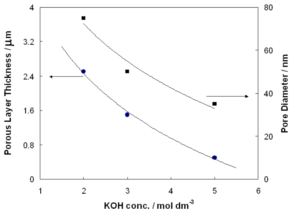
Fig. 8 Plots of the porous layer thickness and mean pore diameter for porous layers formed after a potential sweep at a scan rate of 2.5 \text{ mV s}^{-1} from 0.0 V to 0.825 V, 0.675 V and 0.7 V (SCE) in 2, 3 and 5 mol dm -3 KOH respectively.
