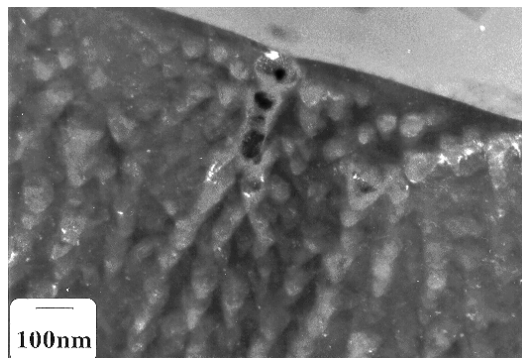
Fig. 3 Dark Field TEM of the porous InP cross-section after a potential sweep from 0.0 V to 0.7 V (SCE) in 5 mol dm -3 KOH showing localized degradation and pore propagation from beneath the etch pit formed in the near-surface layer.
