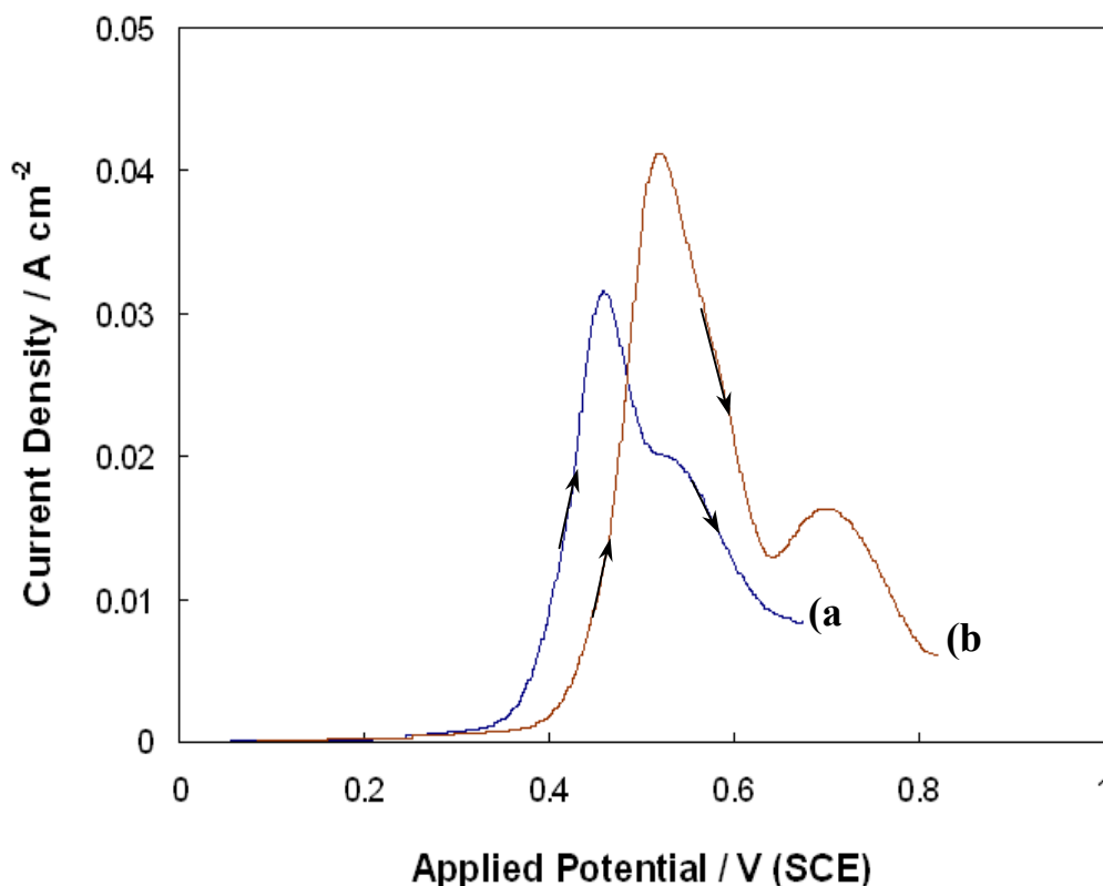
Fig. 5 Linear potential sweeps of InP electrodes in (a) 3 mol dm -3 KOH from 0.0 V to 0.675 V and (b) 2 mol dm -3 KOH from 0.0 V to 0.825 V. The data was acquired at a scan rate of 2.5 mV s -1 .
