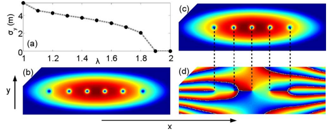
FIG. 1. (Color online) Numerical simulations for a ^{87}\text{Rb} gas of N=10^7 atoms with a_{sc}=4.67 \times 10^{-9} m and trapping frequency \omega = 20\pi \text{ s}^{-1} . (a) Standard deviation \sigma_y of the vortices from the x axis for 1 \leq \lambda \leq 2 . For \lambda \geq 1.9 , the vortices form a linear crystal and \sigma_y=0 . [(b)–(d)] Ground states for a condensate with parameters as above in a trap with aspect ratio of \lambda=2.5 . Each plot spans a range of -36 \mu\text{m} < x < 36 \mu\text{m} and -11 \mu\text{m} < y < 11 \mu\text{m} . (b) Ground-state density for condensate rotating at \Omega=0.7\omega showing six vortices. (c) Ground-state density for condensate rotating at \Omega=0.65\omega showing five vortices. (d) Phase of the cloud shown in (c). The correspondence between the phase singularities and the density dips is indicated.
