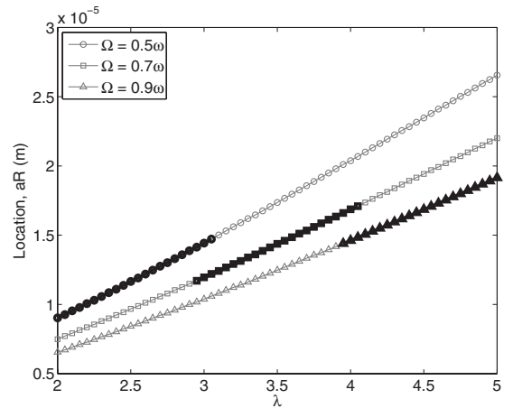
FIG. 5. Distance of outer vortices from the central vortex in the three-vortex case as a function of anisotropy for a range of stirring frequencies. The system parameters are the same as in the two-vortex case.
