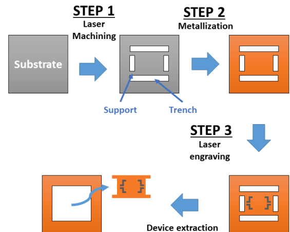
Figure 1. Laser micro-machined fabrication flow.
