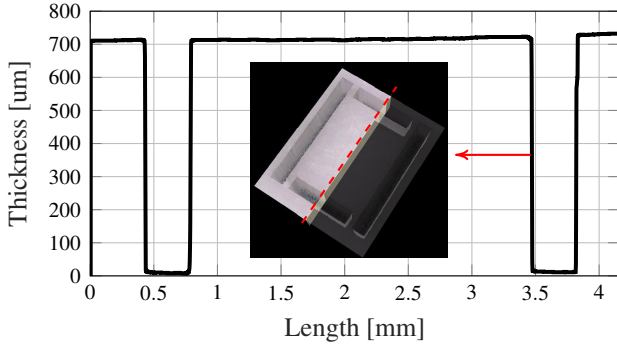
Figure 2. Resonator thickness measured with a digital microscope. Maximum thickness of 732 \mu\text{m} is due to 55 \mu\text{m} separation between the microscope stage and the substrate.
