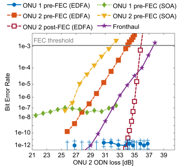
Fig. 5. BER of 10Gb/s PON upstream as a function of ONU 2 ODN loss for the two amplifier node designs and BER of the fronthaul channel as a function of the ODN loss.
