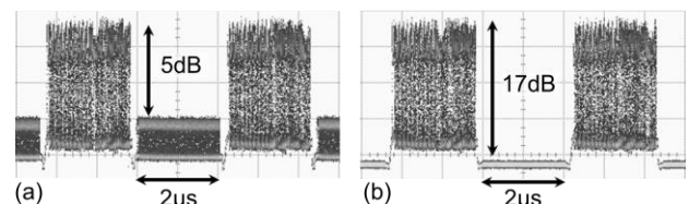
Fig. 6. ONU1 and ONU2 bursts launched in the ODN with 5dB (a) and 17dB (b) power DR.
