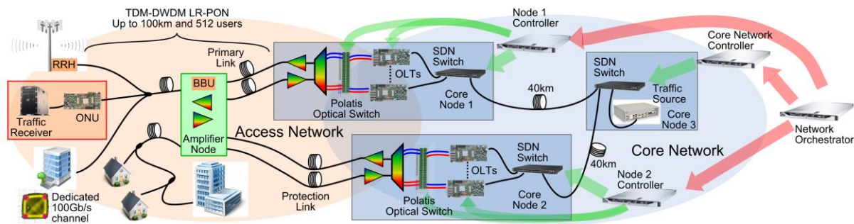
Fig. 1. Network level view of the demonstration.
