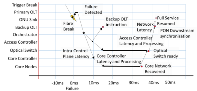
Fig. 11. Breakdown of SDN control plane protection timings.
