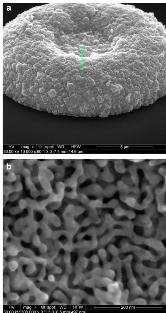
Fig 4 Gold microdisk array modified with nanoporous gold
