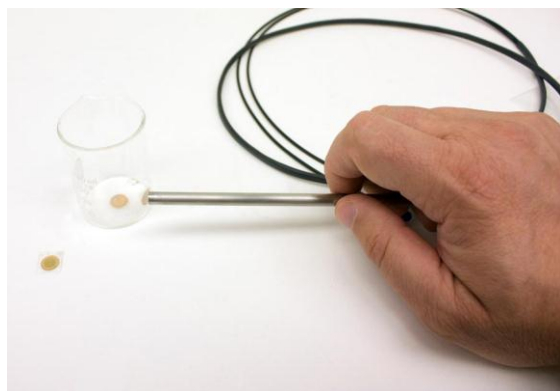
Fig 3: Example of the optical pH 'patch' that can adhere to the inside of a container, while the colour change is observed via an external fibre optic probe (Oceanoptics)
