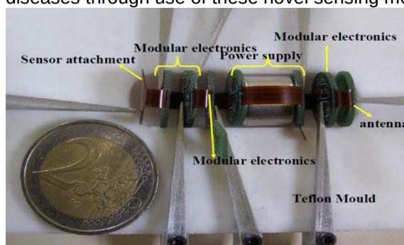
Fig 6: This figure shows the small construction of swallowable capsule, this technology is invaluable to the PATsule project
