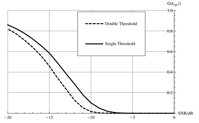
Fig. 8. Plot of the error function with optimised voting rule against SNR for a network of 20 nodes, all of which are certain, with N_s = 200 , \lambda = \lambda_0 = 200 , \lambda_1 = 220 .
