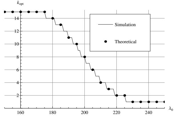
Fig. 4. Plot of optimal voting rule against lower threshold value for a network of 20 nodes, 15 of which are certain, with SNR = -10dB , N_s = 200 , \lambda_1 = \lambda_0 + 20 .
