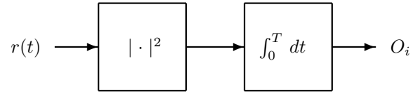
Fig. 1. Illustration of an energy detector.
