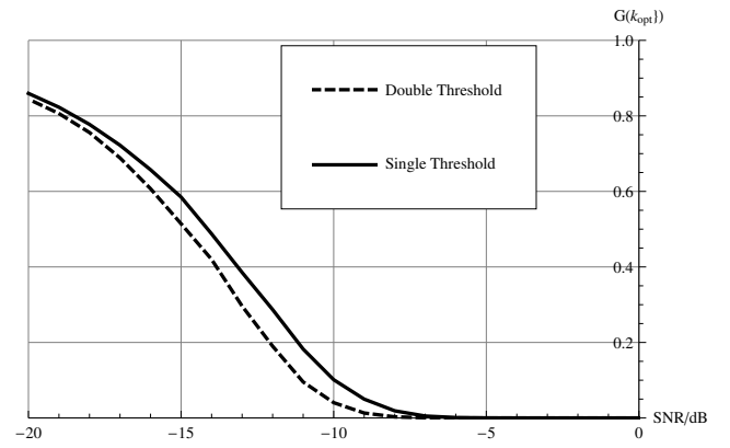
Fig. 9. Plot of the error function with optimised voting rule against SNR for a network of 20 nodes, 15 of which are certain, with N_s = 200 , \lambda = \lambda_0 = 200 , \lambda_1 = 220 .
