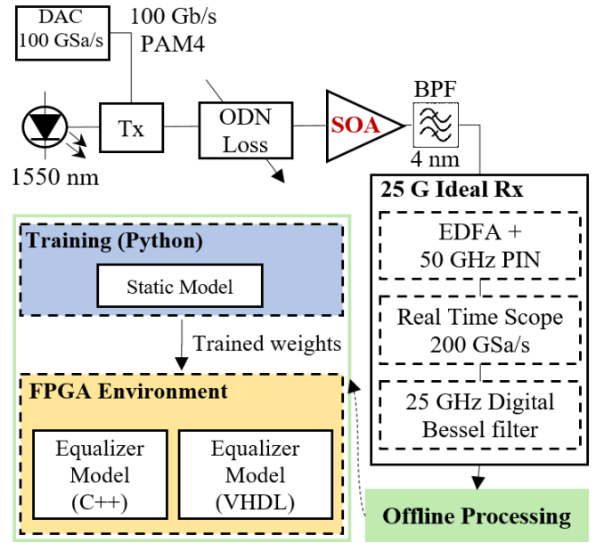
Fig. 2. 100 Gb/s PAM4 back-to-back experimental setup utilizing an SOA preamplifier. DAC: digital-to-analog converter, ODN: optical distribution network, BPF: band-pass filter; SOA: semiconductor optical amplifier; EDFA: erbium-doped fiber amplifier; FPGA: field-programmable gate array
