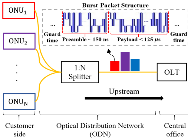
Fig. 1. The upstream transmission architecture in a PON, including an optical line terminal (OLT), an optical distribution network (ODN) containing passive components - such as optical fiber and splitters - and multiple optical network units (ONUs). Additionally, a detailed structure of a burst frame is provided.
