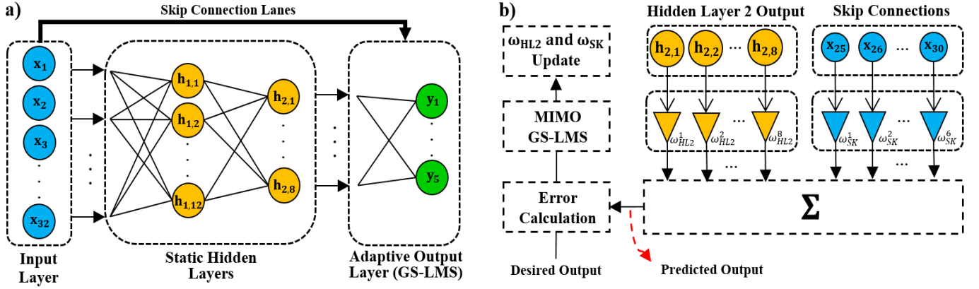
Fig. 3. a) Proposed adaptive FFNN equalizer with skip connection lanes including 32 input taps, two hidden layers with 12 and 8 neurons, respectively, and the adaptive output layer with 5 neurons b) Adaptive training of the FFNN utilizing MIMO GS-LMS algorithm assuming 1 output neuron for simplicity. MIMO GS-LMS: multi-input multi-output gear-shifted least mean square.
