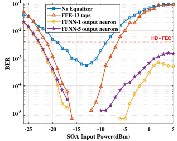
Fig. 5. BER performance, estimated by counting errors over 163k symbols, is compared for the proposed feed-forward neural network (FFNN) equalizer with 1 and 5 output neurons, a conventional 13-tap feed-forward equalizer (FFE), and without equalization in a 100 Gb/s PAM4 PON transmission as the SOA input power increases.
