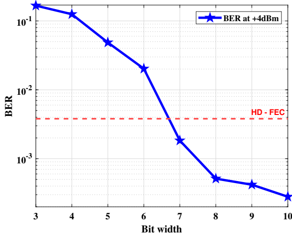
Fig. 4. Quantization analysis of the FFNN equalizer. The BER corresponds to the scenario in which the input power to the SOA is set at +4 dBm.
