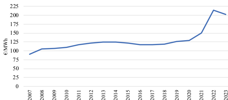
Figure 2. Electricity prices (EU27). Commercial electricity prices in Europe from January 2007 to June 2023. The data is from the Sustainable Energy Authority of Ireland (SEAI).
