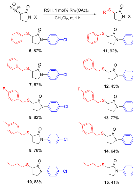
Scheme 3. Rhodium-catalysed S–H insertion reaction to form a library of \alpha -thio-butylolactams.
