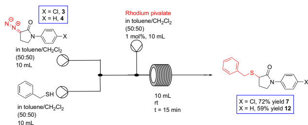
Scheme 5. S-H insertion of 3 and 4 with benzyl mercaptan using rhodium pivalate in continuous flow to form α-thiolactams 7 and 12 .
