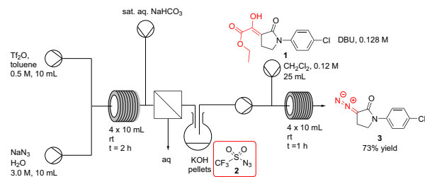
Scheme 1. Telescoped in situ generation of triflyl azide 2 and diazo transfer to form \alpha -diazolactam 3 .
