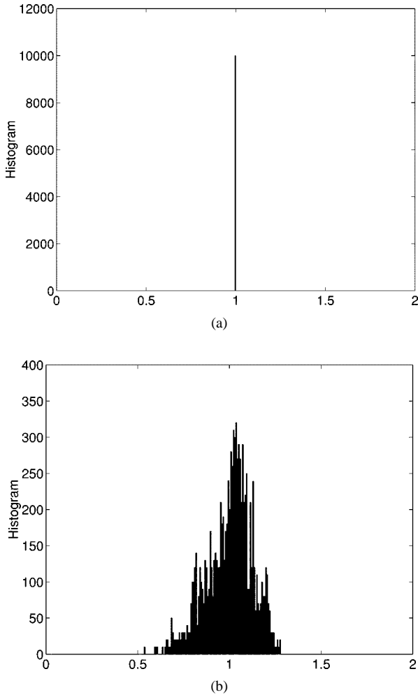
Fig. 3. Samples of \int_0^T g_j^2(t) dt for (a) periodic and (b) chaotic basis functions g_j(t) .
