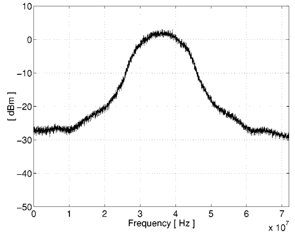
Fig. 19. Output spectrum of an FM-DCSK system. The bit duration is 2 \mu s and the RF channel bandwidth is 17 MHz.
