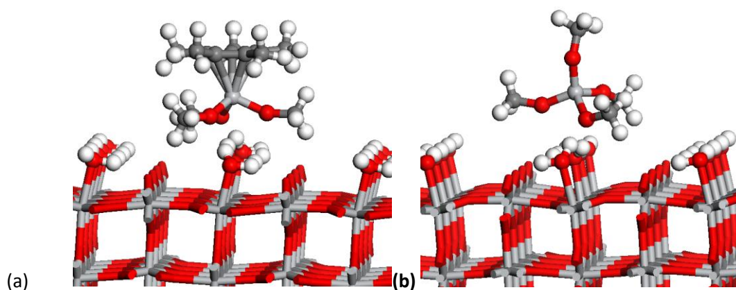
Figure 3: Molecular adsorption of (a) \text{TiCp}^*(\text{OMe})_3 via OMe, (see Figure 6 for adsorption via Cp*) and (b) \text{Ti}(\text{OMe})_4 at the hydrated (1 1 0) surface of \text{TiO}_2 with thicker vacuum. The computed adsorption energies are (a) E_{\text{ads}} = -0.4 eV and (b) E_{\text{ads}} = -0.5 eV.
