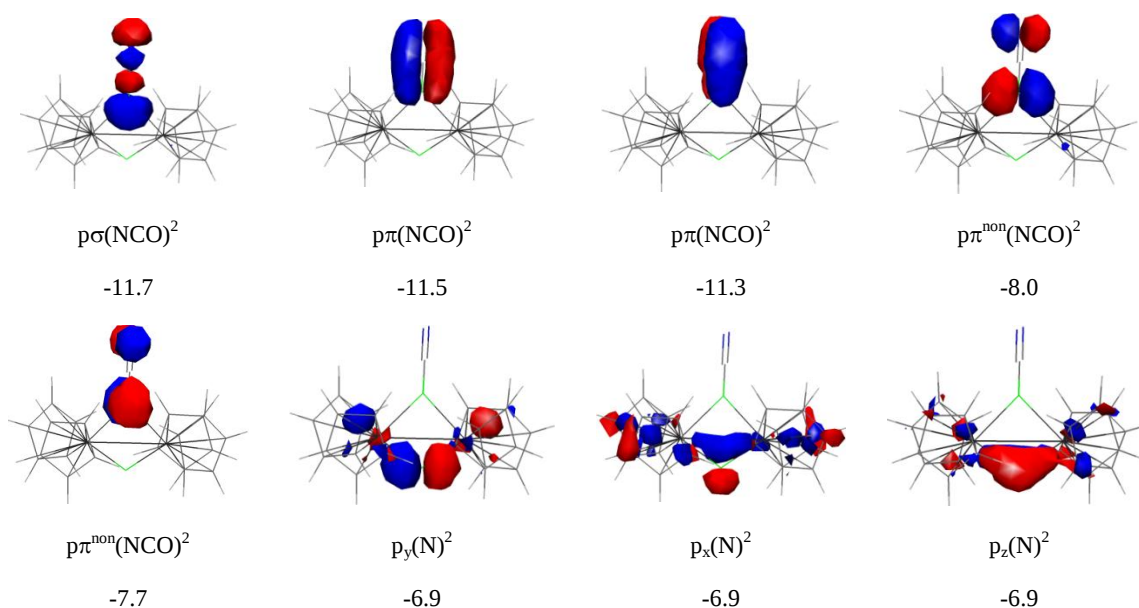
Figure 12 – Selected MOs of the product complex I3, [Hf 2 Cp 2 (NCO)(N)]. The mixing shown in I2 has allowed p\sigma(NN)_2 to be polarised into p(N)_2 , yielding [N]^{3-} , a net gain of one electron by that N atom. Virtual orbitals not shown: p\pi^*(NCO) , p\sigma^*(NCO) . Orbital energies in eV.
