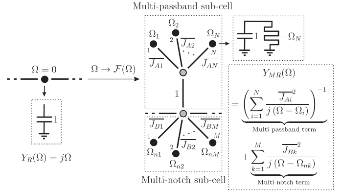
Fig. 1. Normalized coupling-routing diagram of the proposed N -passband/ M -embedded-notch filtering stage after applying the frequency transformation \Omega \rightarrow \mathcal{F}(\Omega) in (1) over a normalized lowpass resonating node (black circles: resonating nodes; grey circles: zero-susceptance non-resonating nodes; continuous lines: couplings; Y_R(\Omega) and Y_{MR}(\Omega) : input admittances of the lowpass resonator and the multi-resonant cell, respectively).
