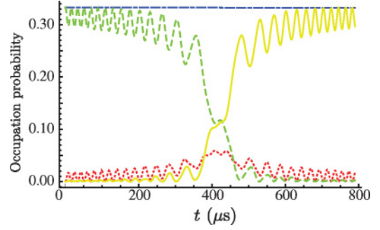
FIG. 3. (Color online) Evolution of the state probabilities |f_i(t)|^2 against the interaction time t (in microseconds) for N_0^I = 10^5 atoms per condensate. Here f_{j,j'}^I = 5 nm, \Omega_I = 27.5 kHz, \chi_{I,\pm 1} = 1.18 kHz, \Delta = 90 kHz, and the two-photon detunings having the functional form \delta_{\pm 1}(t) = 2\Omega_I(1 - \Omega_I t/2) - \omega_t . The trap frequencies are \omega_t = 70 Hz and \omega_z = 500 Hz. The photonic resource is tailored at a wavelength of 702 nm at an angle of 4^\circ off the initial pumping Gaussian beam's axis.
