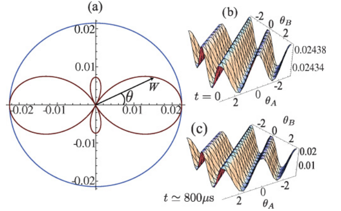
FIG. 7. (Color online) Analysis of the Wigner function for \rho_{AB}(t) . (a) The blue circle shows a projection of the Wigner function on the unit circle for t = 0 , while the red butterfly structure is associated with t \simeq 800 \mu\text{s} , where OAM entanglement has been transferred. (b, c) We plot W(0, \theta_A, 0, \theta_B) at the two instants of time considered for (a). Notice the different vertical-axis scales in the two plots. The visibility of the fringes of interference in the Wigner function is an indication of quantum correlations.
