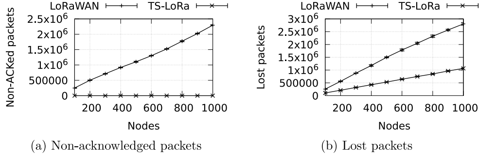
Fig. 10. Number of non-acknowledged and lost packets for variable number of nodes.
