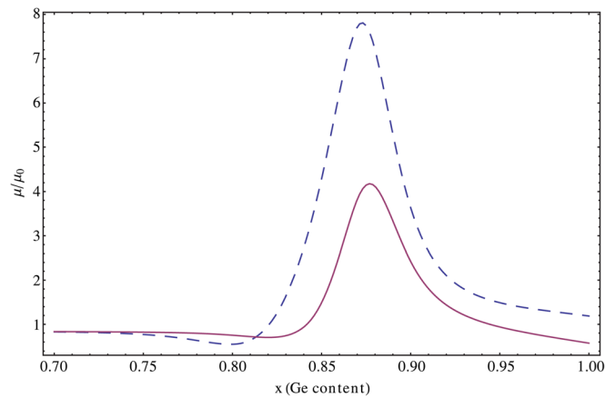
FIG. 10. (Color online) Mobility enhancement of strained SiGe over unstrained SiGe as a function of Ge content, for \varepsilon_{111} = -0.01 (solid line) and \varepsilon_{111} = 0.01 (dashed line), with transport in the [110] direction.
