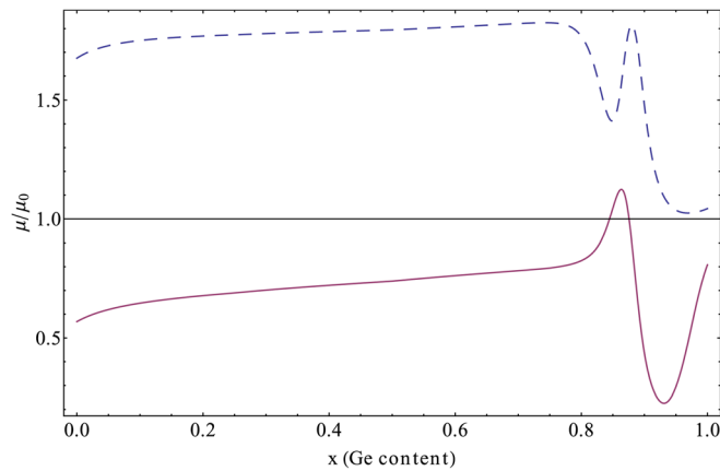
FIG. 8. (Color online) Mobility enhancement of strained SiGe over unstrained SiGe as a function of Ge content, for \varepsilon_{xx} = -0.01 (solid line) and \varepsilon_{xx} = 0.01 (dashed line), with transport in the [100] direction.
