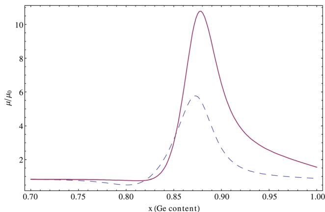
FIG. 9. (Color online) Mobility enhancement of strained SiGe over unstrained SiGe as a function of Ge content, for \varepsilon_{111} = -0.01 (solid line) and \varepsilon_{111} = 0.01 (dashed line), with transport in the [110] direction.
