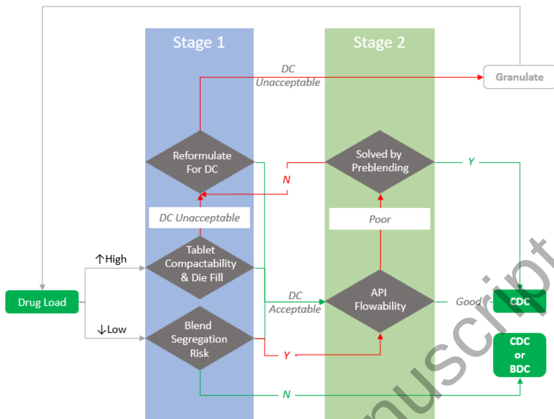
Figure 4: Proposal for deciding for choosing batch or continuous manufacturing processes
