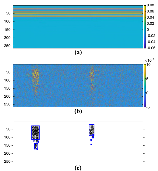
Fig. 5 a Raw echo profile matrix. b Echo profile matrix after column-wise subtraction. c Echo profile matrix after binarisation and segmentation; blue-coloured bounding boxes indicate detected strokes
