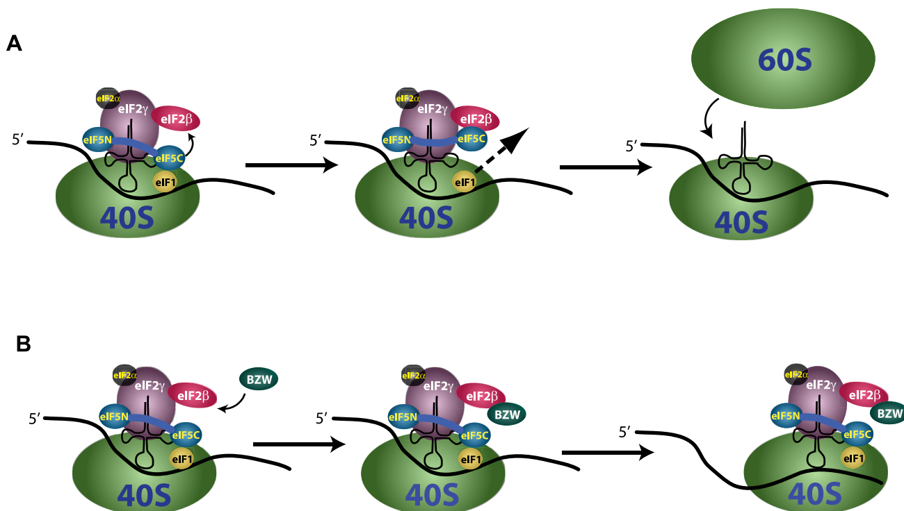
Fig 4. A model for the molecular interactions likely to account for the effect of BZW1 and BZW2 on stringency of start codon selection. During scanning, when the 40S subunit is in the open conformation, eIF1 is bound near the P-site and monitors the interaction between tRNA i Met and nucleotide triplets in the mRNA. The eIF5 C-terminal domain is loosely bound to eIF1 working as a lid to prevent the premature release of eIF1 from the PIC. (A) Under low BZW levels, the eIF2β N-terminal domain and eIF5 C-terminal domain occasionally interact pulling eIF5 away from eIF1, allowing its looser association with the PIC. The lower affinity of eIF1 for the PIC facilitates more frequent initiation at near-cognate or suboptimal AUG codons. (B) BZW, perhaps through its C-terminal HEAT domain, binds to the eIF2β N-terminal domain. When levels of BZW protein are high this interaction is favored, and this prevents interaction between eIF2β and eIF5. This leaves the “lid” on eIF1 closed, essentially increasing its effective concentration on the PIC and this enhances stringency of start codon selection, resulting in lower frequency of initiation at near-cognate start codons or poor context AUG triplets, including the start codons of BZW genes, with ribosome continuing to scan in the 3' direction for a better start codon.
