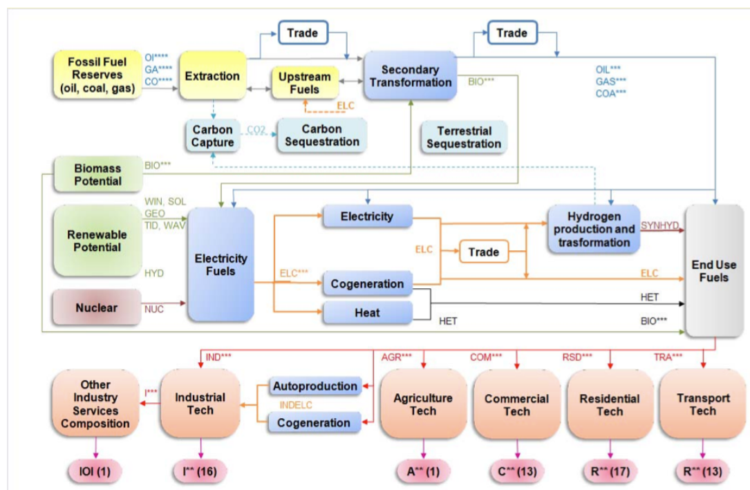
Appendix Figure 2 - Schematic of processes and commodities in TIMES (source: (Ó Gallachóir et al., 2012))
