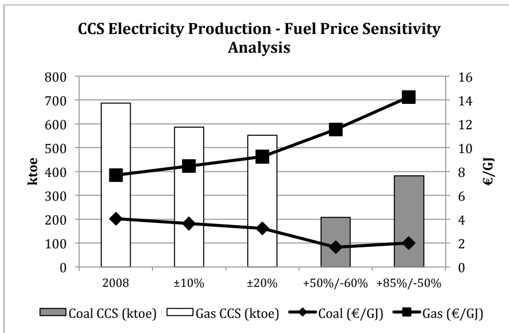
Figure 6-6 - Installed CCS capacity Irish TIMES results for sensitivity analysis of fuel price costs
