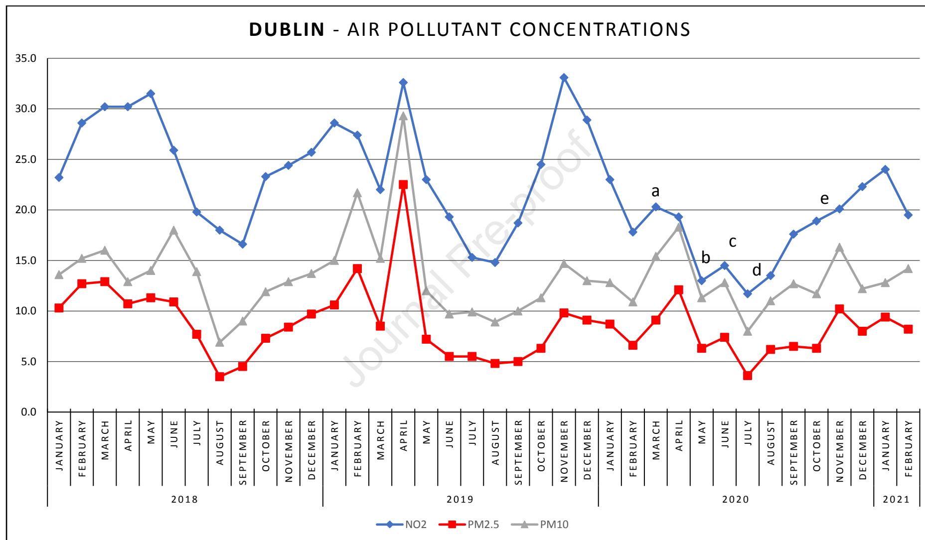
Figure 1 Graph of average concentration of NO 2 , PM 2.5 and PM 10 for each month of the study period; a: 2km restrictions introduced, b: 5km restrictions introduced, c: 20km restrictions introduced, d: cross-country travel allowed, e: cross-country restrictions re-imposed.
