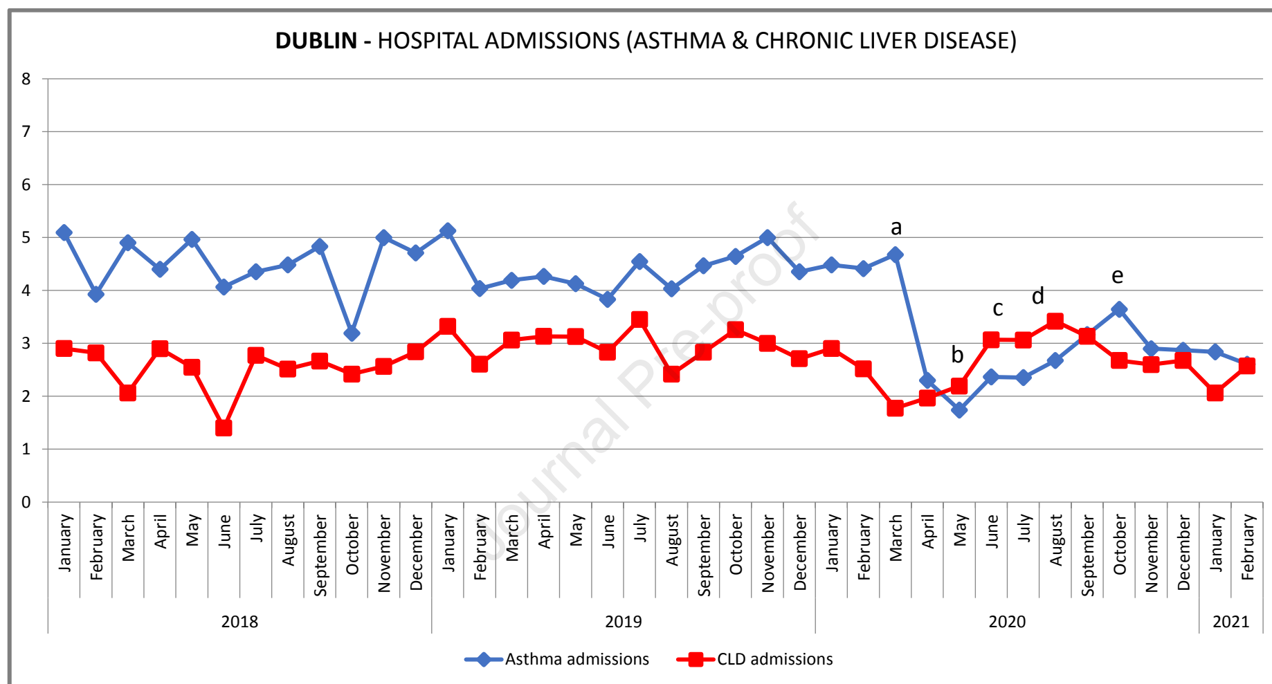
Figure 2 Graph of average daily hospital admissions for asthma and chronic liver disease for each month of the study period; a: 2km restrictions introduced, b: 5km restrictions introduced, c: 20km restrictions introduced, d: cross-country travel allowed, e: cross-country restrictions re-imposed.
