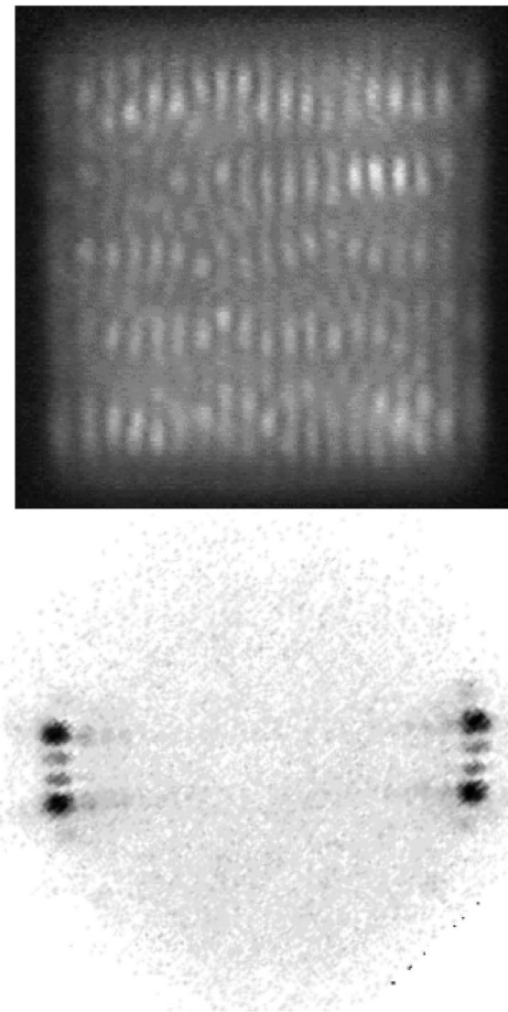
FIG. 2. Near field (top) and far field (bottom) of a single frequency standing wave of the laser intensity. The laser aperture is 15 \times 15 \mu\text{m}^2 . The spatial wavelength of the intensity of this pattern is approximately 0.75 \mu\text{m} and the corresponding divergence in air is 65^\circ full angle.
