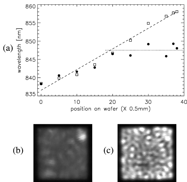
FIG. 3. (a) Laser wavelength as a function of position for both small and large VCSELs. Squares correspond to small Fresnel number lasers and dots to large Fresnel number lasers. The dashed line is a fit to the nearly linear variation of cavity resonance wavelength, the dotted line a fit to the broad area laser wavelength. (b) Near field of negatively detuned laser close to threshold. (c) Near field of negatively detuned laser at twice threshold.
