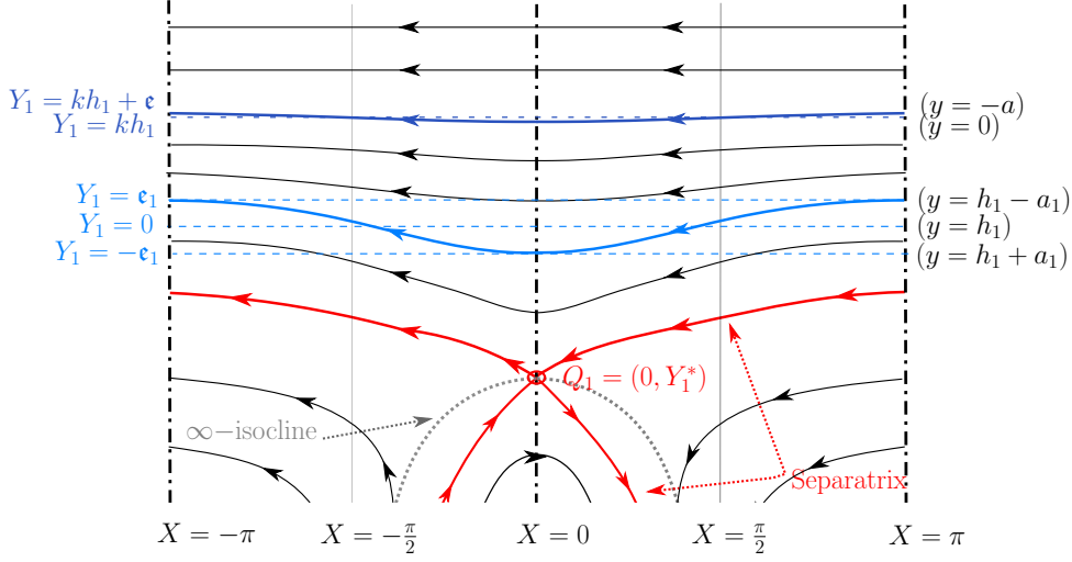
Figure 6: Phase portrait of the upper-fluid layer when A = 1 . The dotted grey line \cdots represents the \infty -isocline, while the dotted-dashed lines \cdots represent the 0-isoclines. The surface wave profile (—) has mean-water level Y_1 = 0 , corresponding to y = h_1 . The internal wave profile (—) has mean water level Y = kh_1 , corresponding to y = 0 . Note (cf. Remark 11) that the streamline representing the surface wave lies beneath that of the internal wave in this phase portrait.
