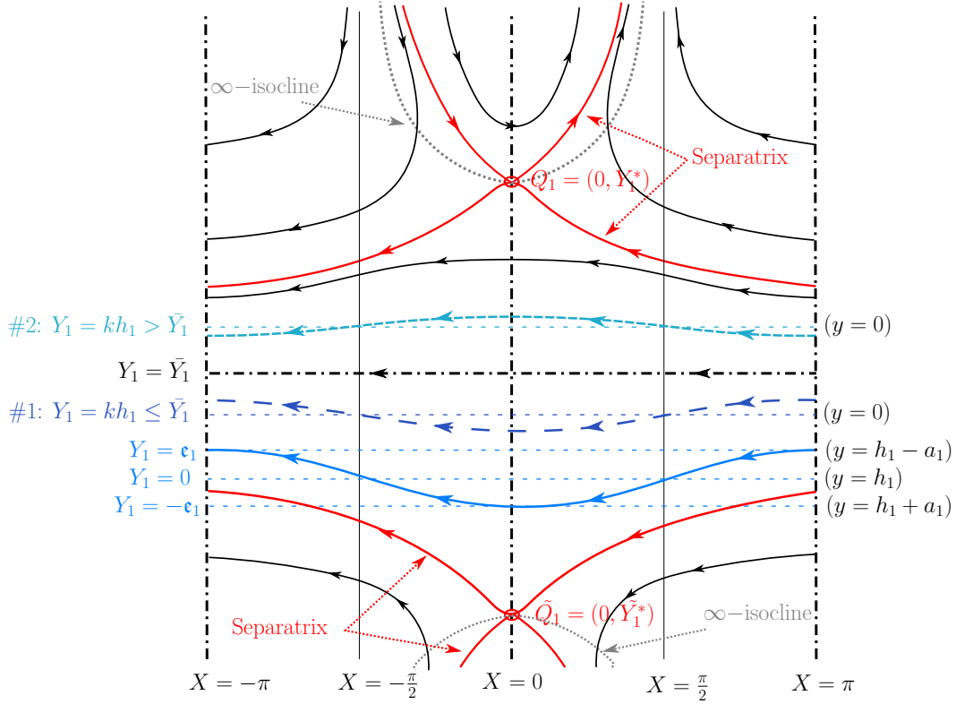
Figure 8: Phase portrait for the upper-fluid layer when A > 1 . The dotted grey lines \cdots represent the \infty -isoclines, with the dotted-dashed lines \cdots representing the 0-isoclines. The surface wave profile (—) has mean-water level Y_1 = 0 , corresponding to y = h_1 . The internal wave profile is illustrated for two differing values of the mean water level Y = kh_1 , corresponding to y = 0 : kh_1 \leq \bar{Y}_1 in Case 1 (—), whereas kh_1 > \bar{Y}_1 for Case 2 (---). Note (cf. Remark 11) that the streamline representing the surface wave lies beneath that of the internal wave in this phase portrait.
