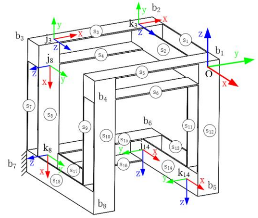
Fig. 6 Discretization of the structure of the compliant elements.
