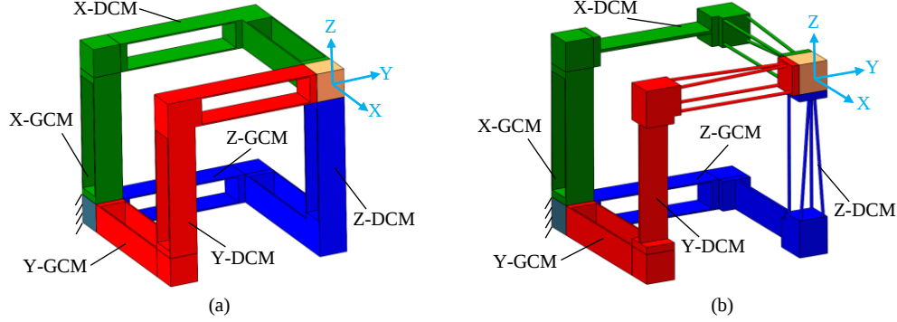
Fig. 5 Two asymmetric XYZ compliant parallel mechanisms: (a) Asymmetric design for Case-1, and (b) Asymmetric design for Case-2 ( X-GCM and X-DCM are shown in green, Y-GCM and Y-DCM are shown in red, Z-GCM and Z-DCM are shown in blue, IRM is shown in orange, FRM is shown in grey).
