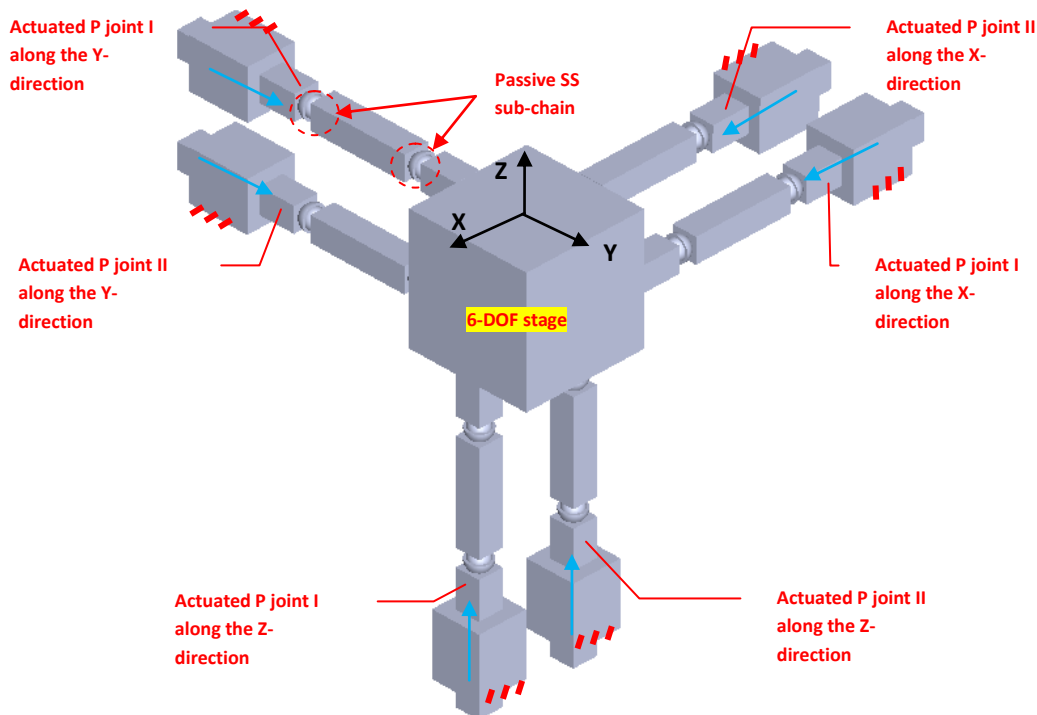
Fig. 9 A 6-PSS parallel mechanism
