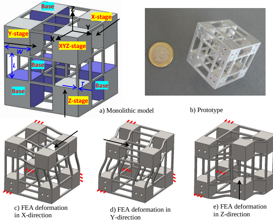
Fig. 5 A monolithic decoupled 3-PPPR XYZ CPM with extended life composed of 12 identical WBBCM3-1s
