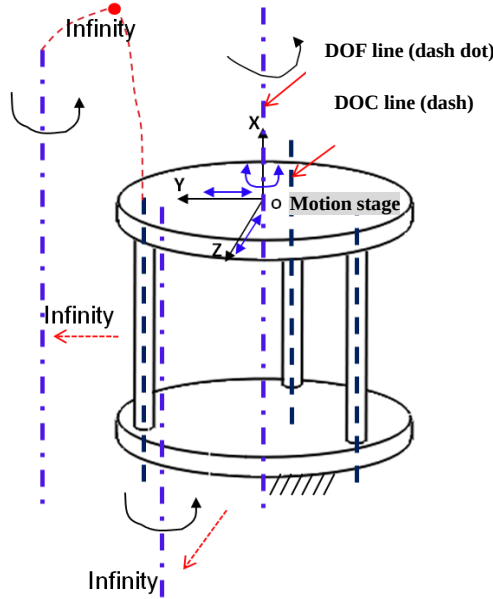
Fig. 1 A WBBCM composed of three independent wire beams: spatial three-beam module
