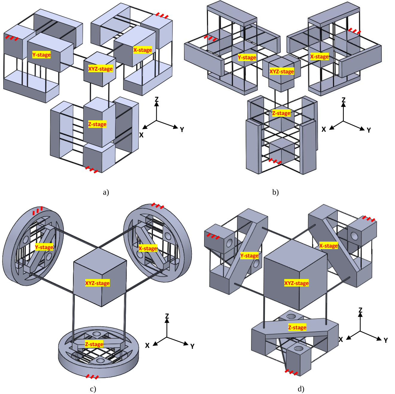
Fig. 8 Other 3-PPRR XYZ CPMs
