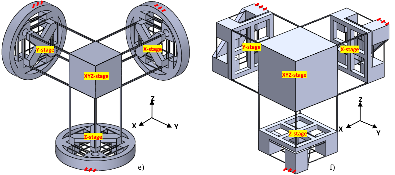
Fig. 6 Other 3-PPRR XYZ CPMs (continued)
