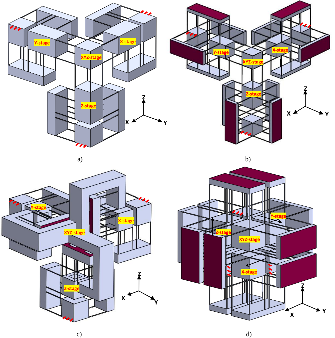
Fig. 6 Other 3-PPPR XYZ CPMs
