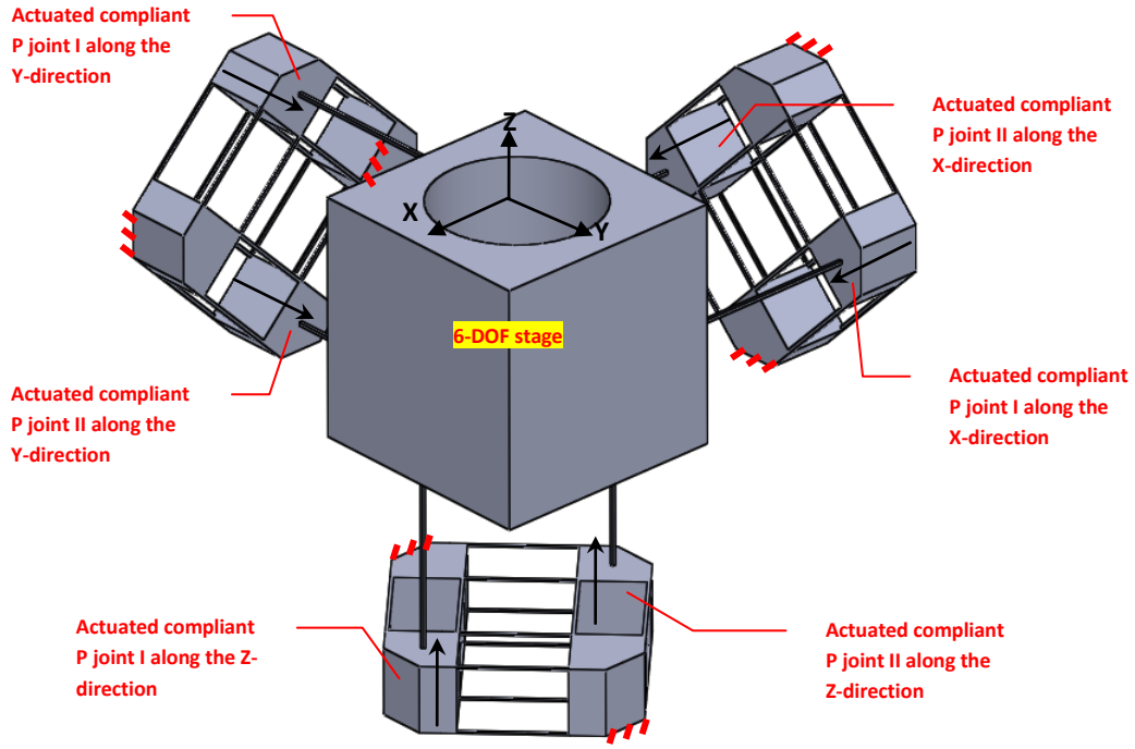
Fig. 10 A 6-DOF CPM
