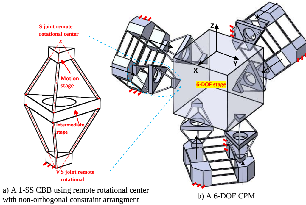
Fig. 11 Another type of 6-DOF CPM
