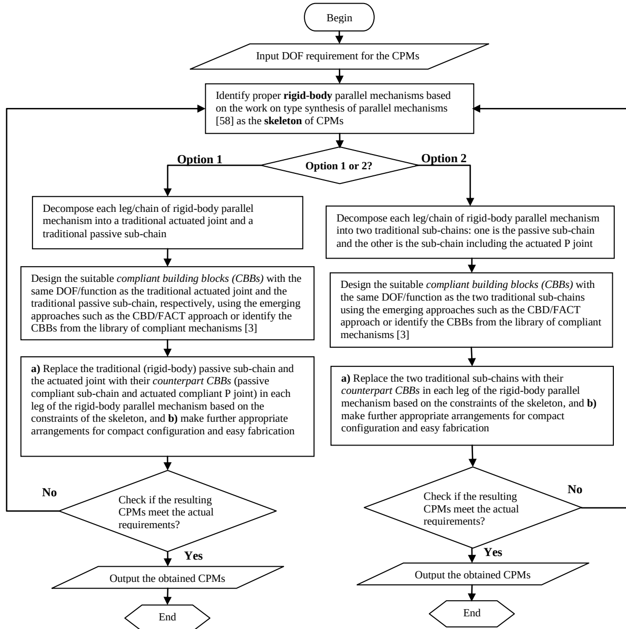
Fig. 2 Flow chart for the building block based PRBM method
