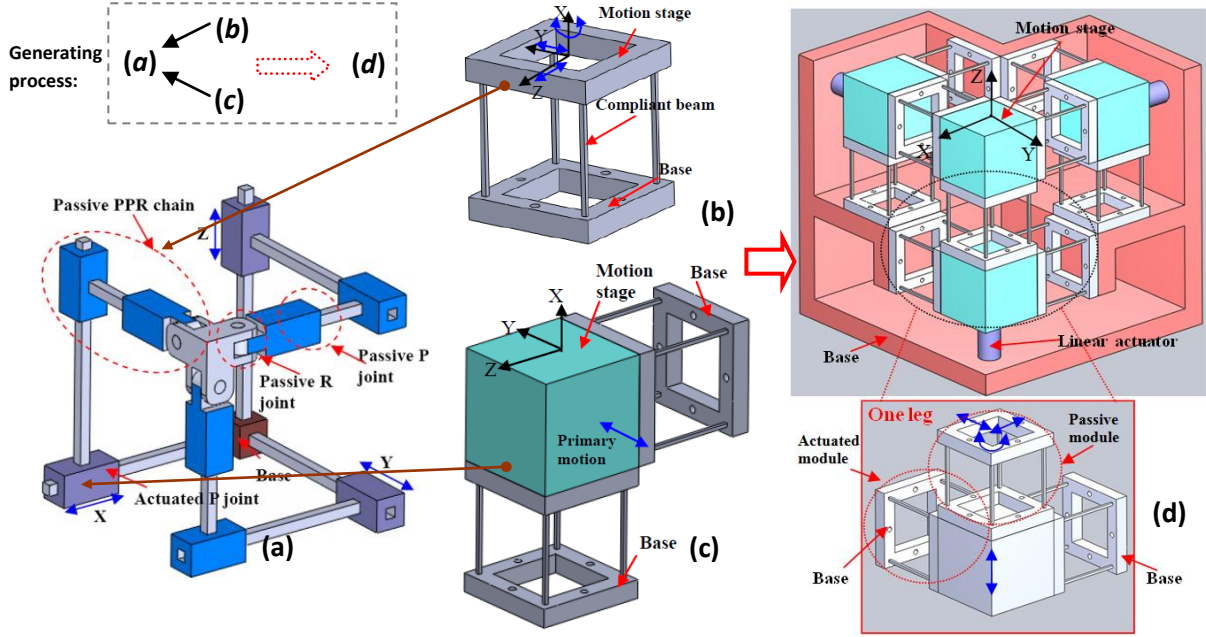
Fig. 4 The generating process of a decoupled 3-PPPR XYZ CPM: (a) A kinematically decoupled 3-PPPR TPM; (b) WBBCM3-1; (c) WBBCM4-1 composed two identical WBBCM3-1 in parallel; (d) A decoupled XYZ CPM composed of identical WBBCM3-1s
