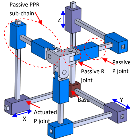
(b) 3- PPR TPM
