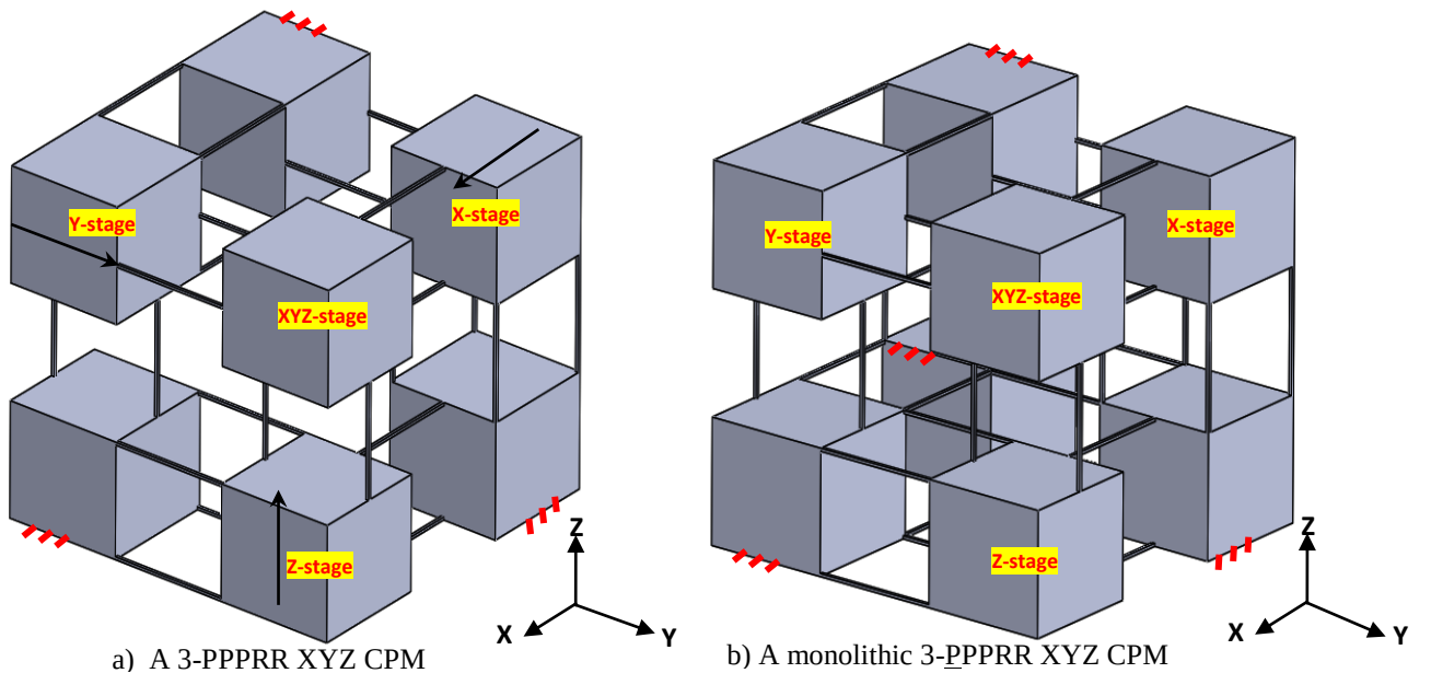
Fig. 7 3-PPRR XYZ CPMs
